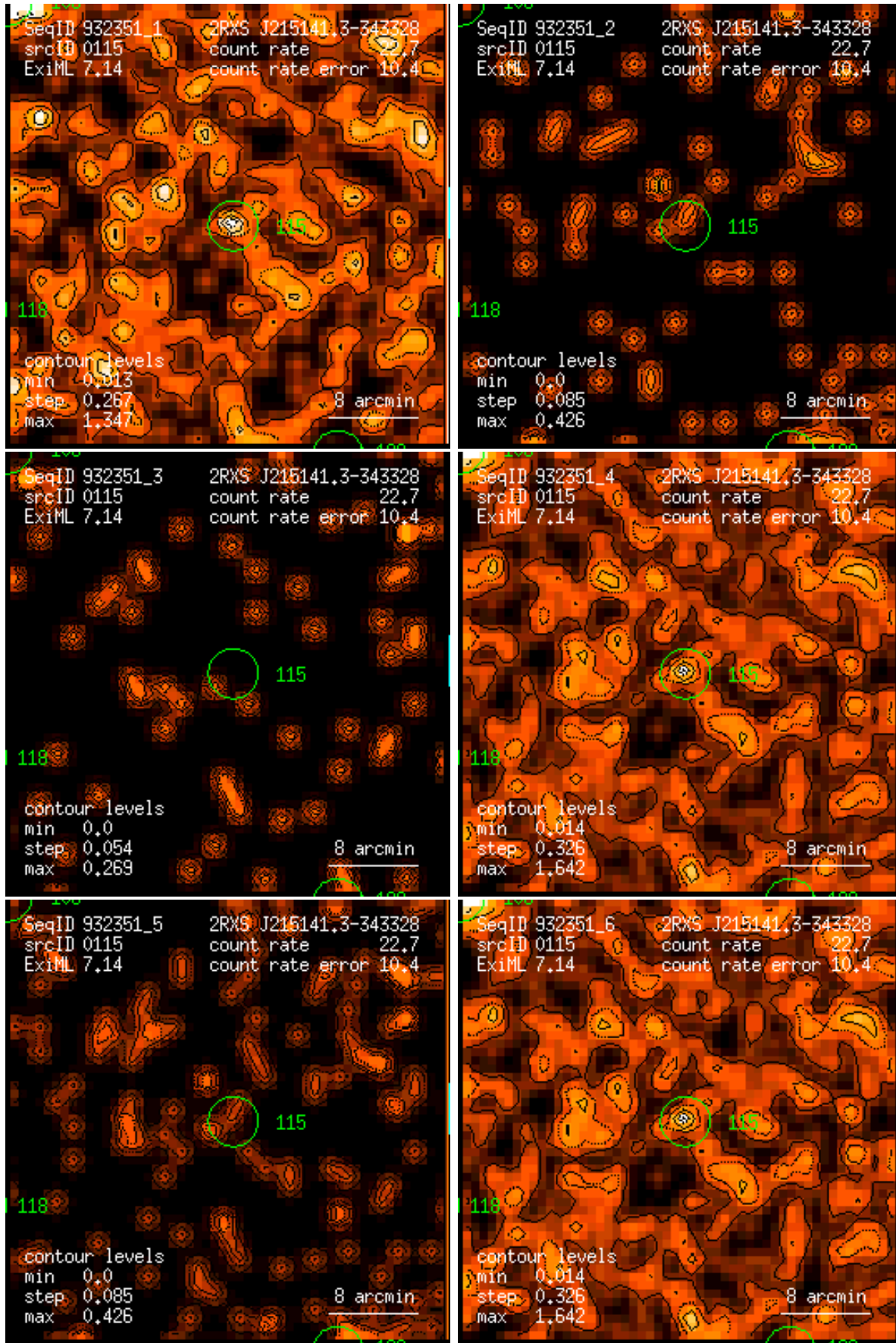
Figure 115: RASS 932351: detection 0115: band rate images, Gaussian filter: (1) PSPC channels 11 – 41, (2) 52 – 90, (3) 91 – 201, (4) 11 – 235, (5) 52 – 201, (6) 11 – 201. Broad band rates in counts/ks. Band rate contour levels in counts/ks/arcmin 2 .
