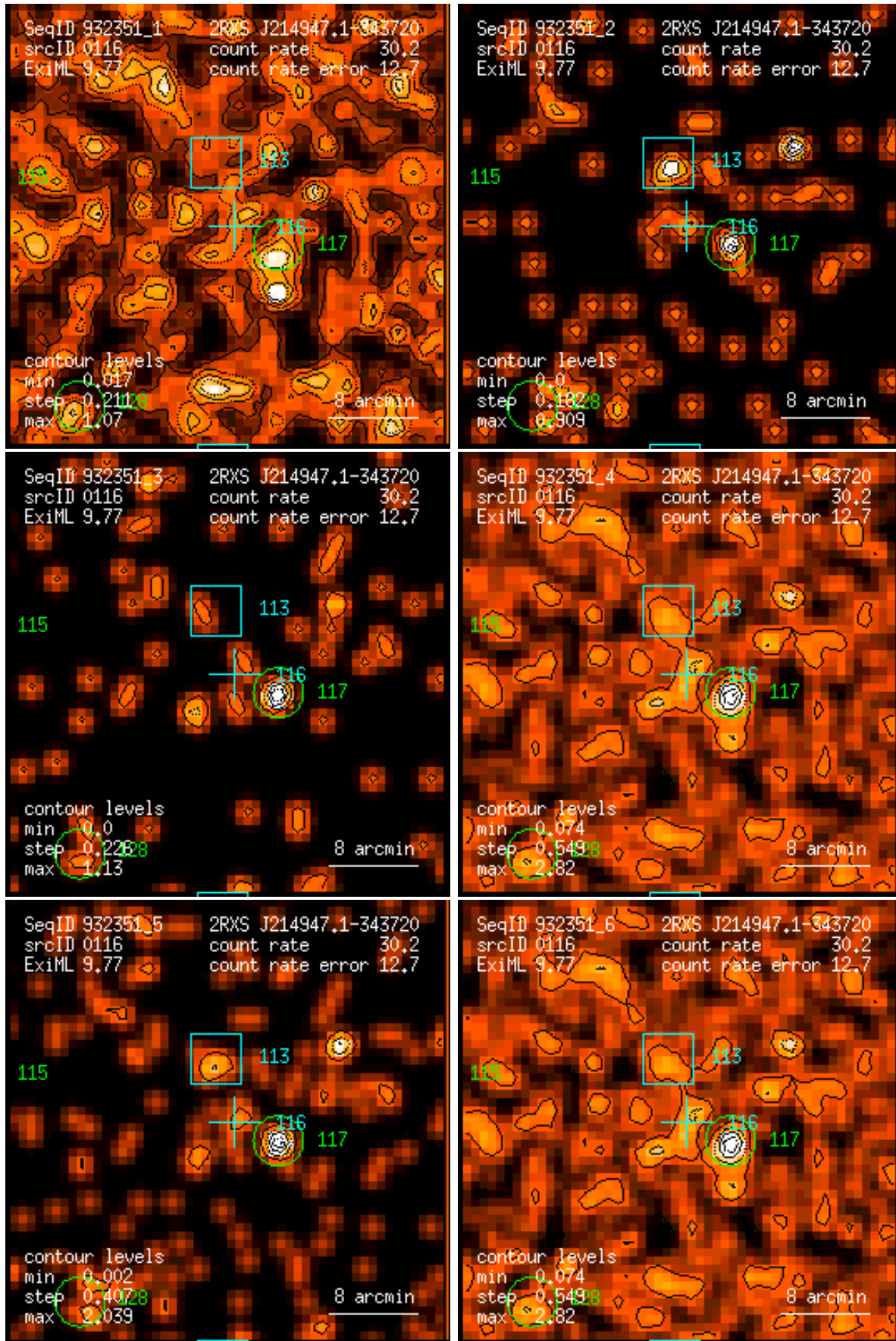
Figure 116: RASS 932351: detection 0116: band rate images, Gaussian filter: (1) PSPC channels 11 – 41, (2) 52 – 90, (3) 91 – 201, (4) 11 – 235, (5) 52 – 201, (6) 11 – 201. Broad band rates in counts/ks. Band rate contour levels in counts/ks/arcmin 2 .
