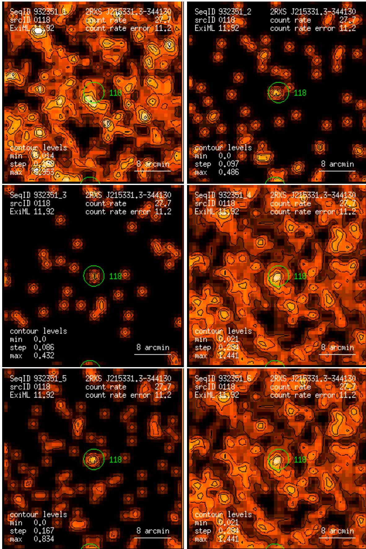
Figure 118: RASS 932351: detection 0118: band rate images, Gaussian filter: (1) PSPC channels 11 – 41, (2) 52 – 90, (3) 91 – 201, (4) 11 – 235, (5) 52 – 201, (6) 11 – 201. Broad band rates in counts/ks. Band rate contour levels in counts/ks/arcmin 2 .
