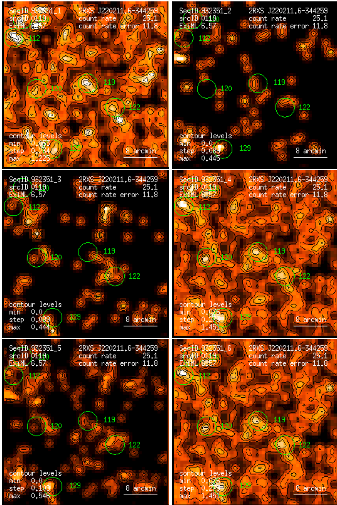
Figure 119: RASS 932351: detection 0119: band rate images, Gaussian filter: (1) PSPC channels 11 – 41, (2) 52 – 90, (3) 91 – 201, (4) 11 – 235, (5) 52 – 201, (6) 11 – 201. Broad band rates in counts/ks. Band rate contour levels in counts/ks/arcmin 2 .
