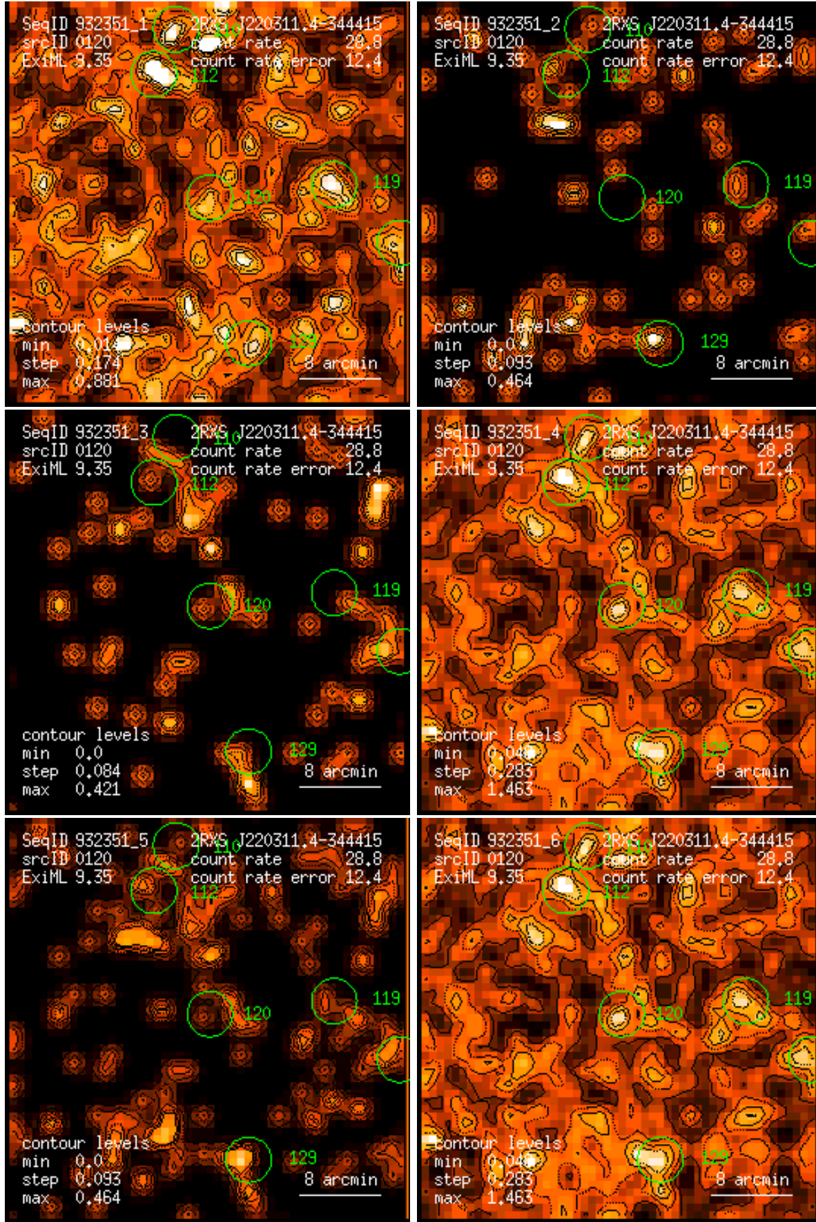
Figure 120: RASS 932351: detection 0120: band rate images, Gaussian filter: (1) PSPC channels 11 – 41, (2) 52 – 90, (3) 91 – 201, (4) 11 – 235, (5) 52 – 201, (6) 11 – 201. Broad band rates in counts/ks. Band rate contour levels in counts/ks/arcmin 2 .
