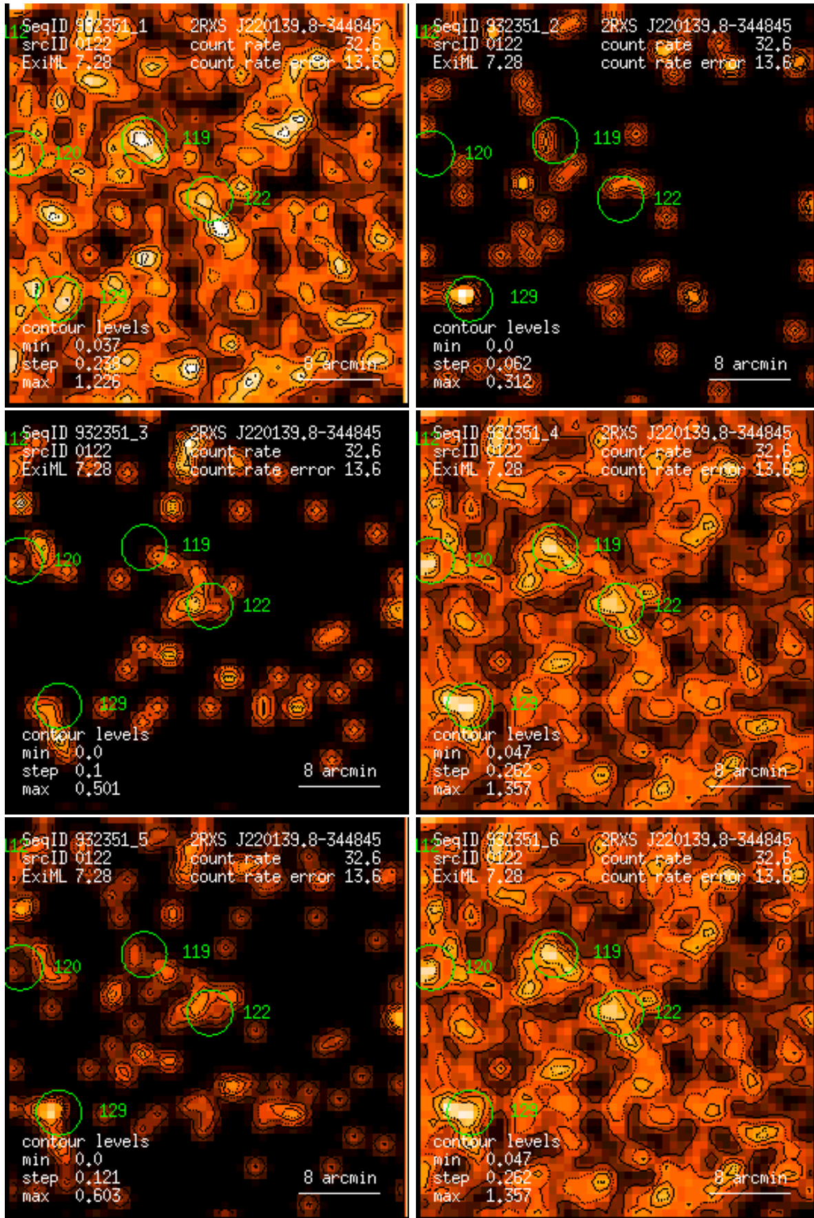
Figure 122: RASS 932351: detection 0122: band rate images, Gaussian filter: (1) PSPC channels 11 – 41, (2) 52 – 90, (3) 91 – 201, (4) 11 – 235, (5) 52 – 201, (6) 11 – 201. Broad band rates in counts/ks. Band rate contour levels in counts/ks/arcmin 2 .
