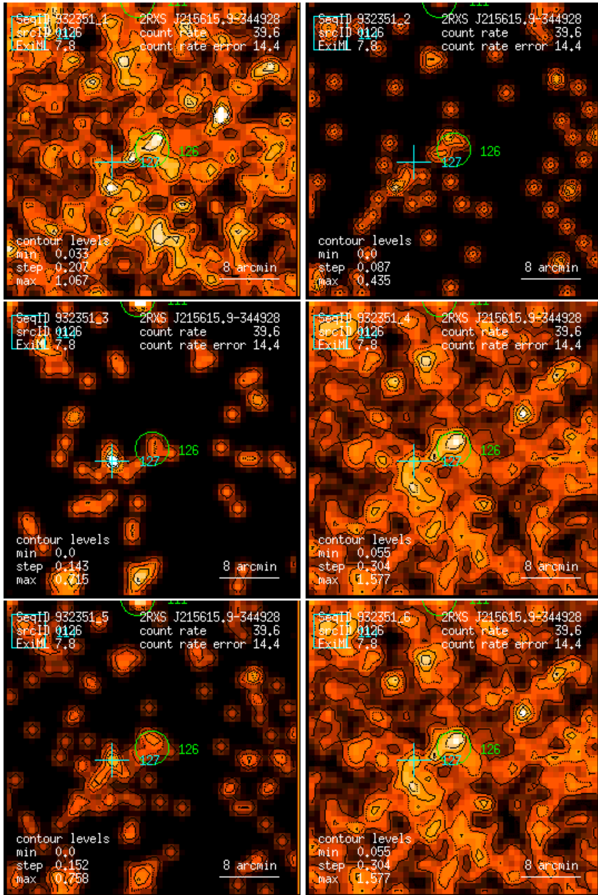
Figure 126: RASS 932351: detection 0126: band rate images, Gaussian filter: (1) PSPC channels 11 – 41, (2) 52 – 90, (3) 91 – 201, (4) 11 – 235, (5) 52 – 201, (6) 11 – 201. Broad band rates in counts/ks. Band rate contour levels in counts/ks/arcmin 2 .
