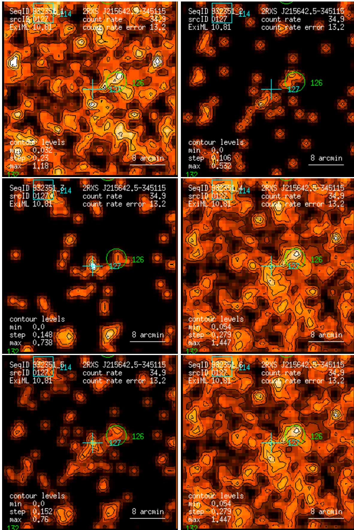
Figure 127: RASS 932351: detection 0127: band rate images, Gaussian filter: (1) PSPC channels 11 – 41, (2) 52 – 90, (3) 91 – 201, (4) 11 – 235, (5) 52 – 201, (6) 11 – 201. Broad band rates in counts/ks. Band rate contour levels in counts/ks/arcmin 2 .
