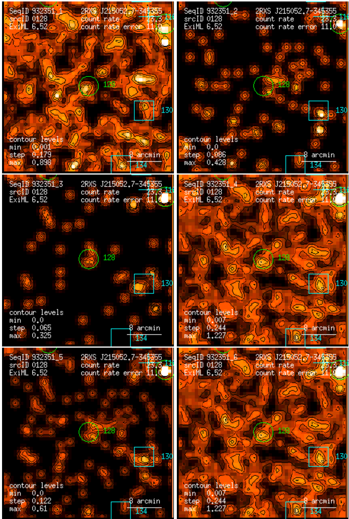
Figure 128: RASS 932351: detection 0128: band rate images, Gaussian filter: (1) PSPC channels 11 – 41, (2) 52 – 90, (3) 91 – 201, (4) 11 – 235, (5) 52 – 201, (6) 11 – 201. Broad band rates in counts/ks. Band rate contour levels in counts/ks/arcmin 2 .
