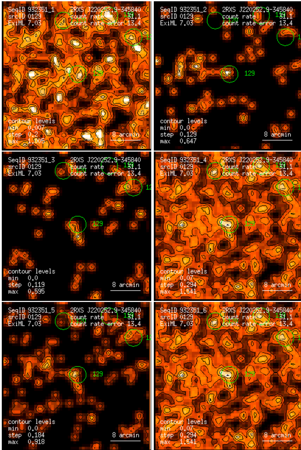
Figure 129: RASS 932351: detection 0129: band rate images, Gaussian filter: (1) PSPC channels 11 – 41, (2) 52 – 90, (3) 91 – 201, (4) 11 – 235, (5) 52 – 201, (6) 11 – 201. Broad band rates in counts/ks. Band rate contour levels in counts/ks/arcmin 2 .
