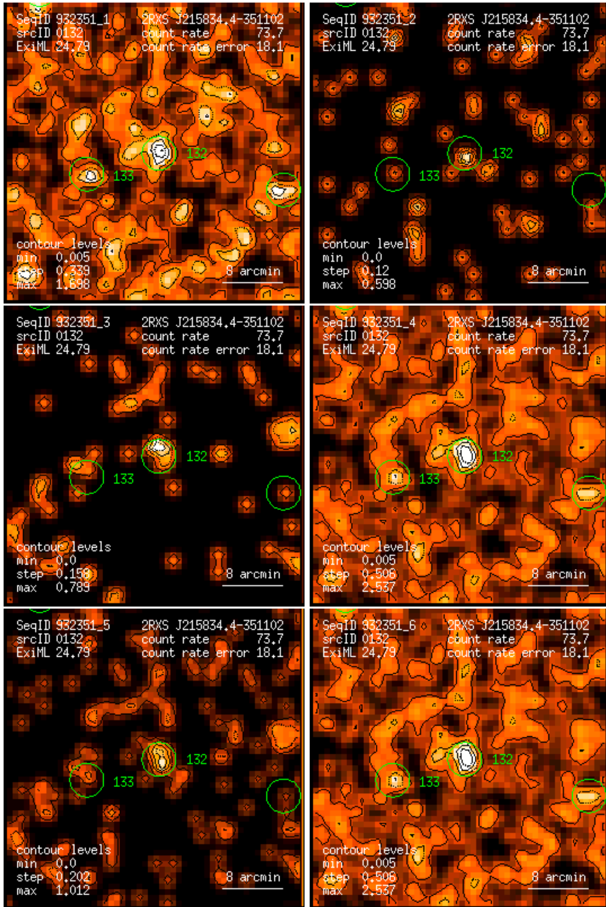
Figure 132: RASS 932351: detection 0132: band rate images, Gaussian filter: (1) PSPC channels 11 – 41, (2) 52 – 90, (3) 91 – 201, (4) 11 – 235, (5) 52 – 201, (6) 11 – 201. Broad band rates in counts/ks. Band rate contour levels in counts/ks/arcmin 2 .
