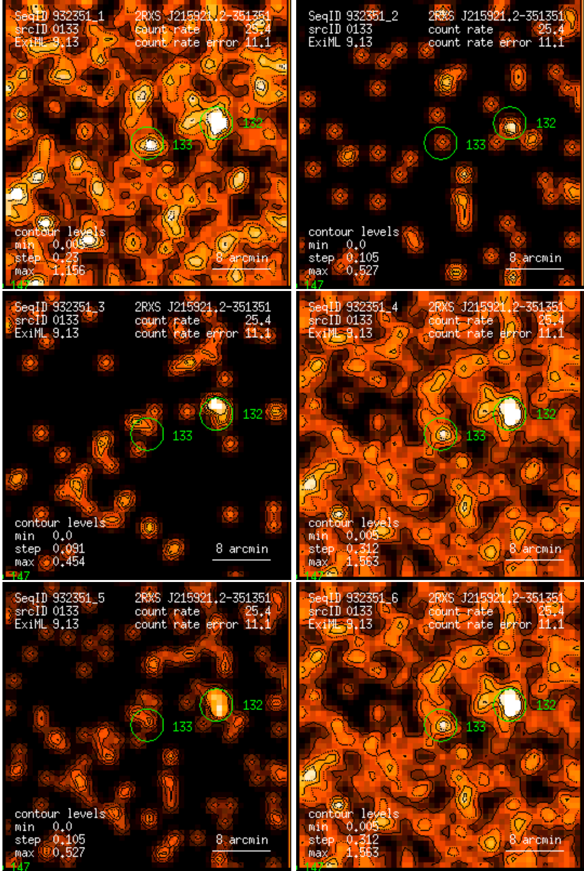
Figure 133: RASS 932351: detection 0133: band rate images, Gaussian filter: (1) PSPC channels 11 – 41, (2) 52 – 90, (3) 91 – 201, (4) 11 – 235, (5) 52 – 201, (6) 11 – 201. Broad band rates in counts/ks. Band rate contour levels in counts/ks/arcmin 2 .
