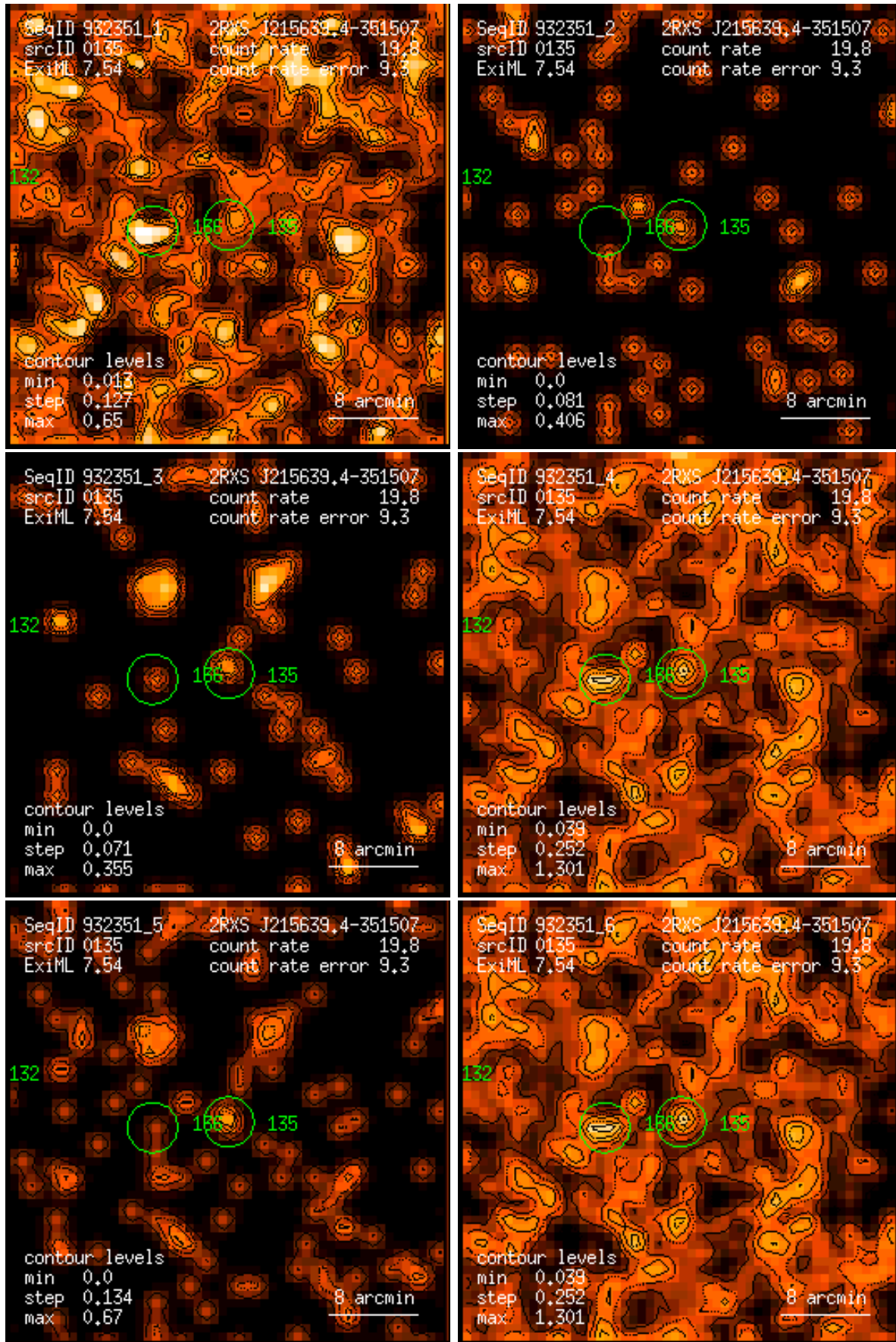
Figure 135: RASS 932351: detection 0135: band rate images, Gaussian filter: (1) PSPC channels 11 – 41, (2) 52 – 90, (3) 91 – 201, (4) 11 – 235, (5) 52 – 201, (6) 11 – 201. Broad band rates in counts/ks. Band rate contour levels in counts/ks/arcmin 2 .
