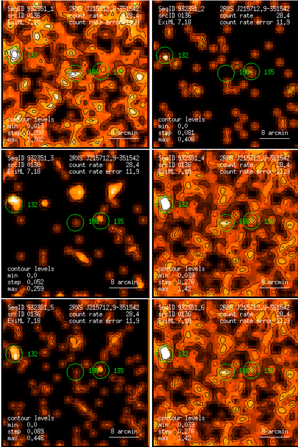
Figure 136: RASS 932351: detection 0136: band rate images, Gaussian filter: (1) PSPC channels 11 – 41, (2) 52 – 90, (3) 91 – 201, (4) 11 – 235, (5) 52 – 201, (6) 11 – 201. Broad band rates in counts/ks. Band rate contour levels in counts/ks/arcmin 2 .
