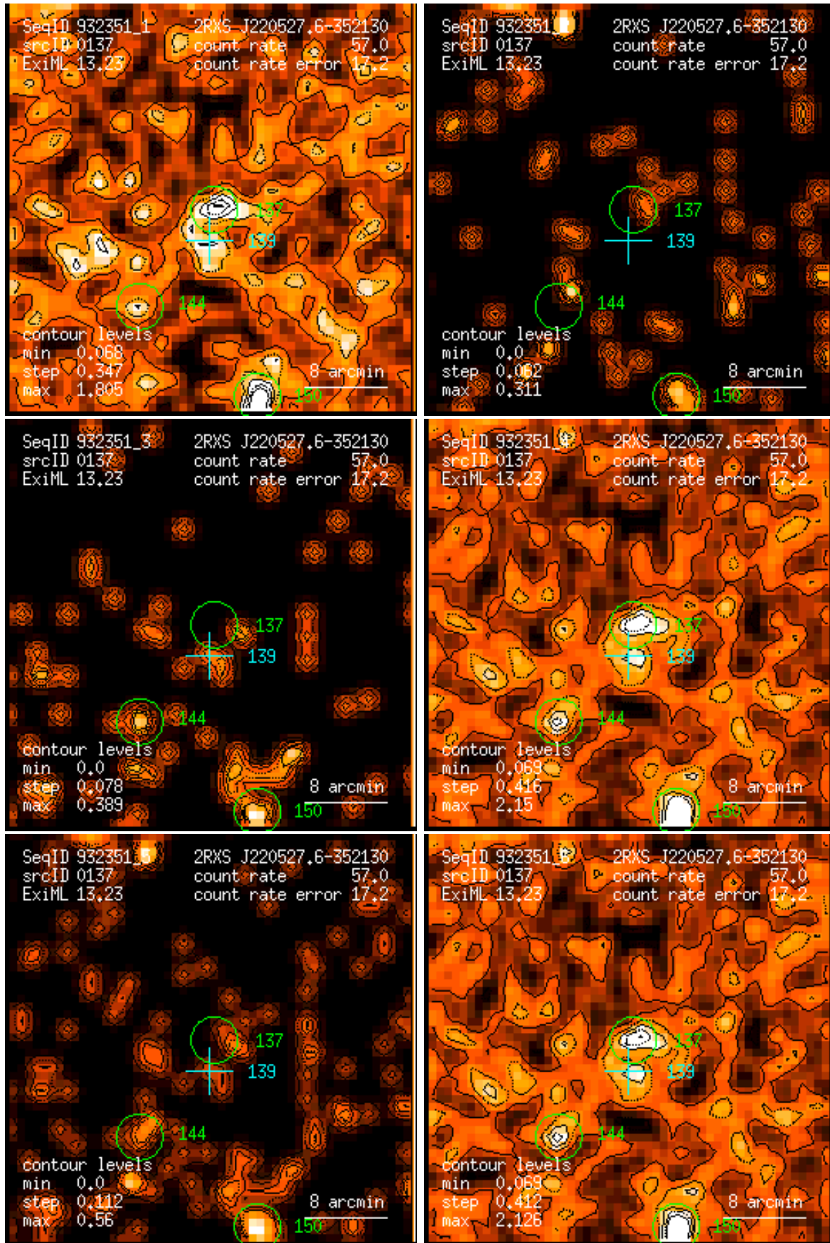
Figure 137: RASS 932351: detection 0137: band rate images, Gaussian filter: (1) PSPC channels 11 – 41, (2) 52 – 90, (3) 91 – 201, (4) 11 – 235, (5) 52 – 201, (6) 11 – 201. Broad band rates in counts/ks. Band rate contour levels in counts/ks/arcmin 2 .
