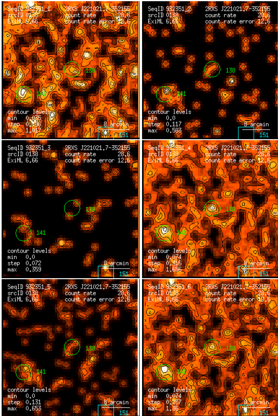
Figure 138: RASS 932351: detection 0138: band rate images, Gaussian filter: (1) PSPC channels 11 – 41, (2) 52 – 90, (3) 91 – 201, (4) 11 – 235, (5) 52 – 201, (6) 11 – 201. Broad band rates in counts/ks. Band rate contour levels in counts/ks/arcmin 2 .
