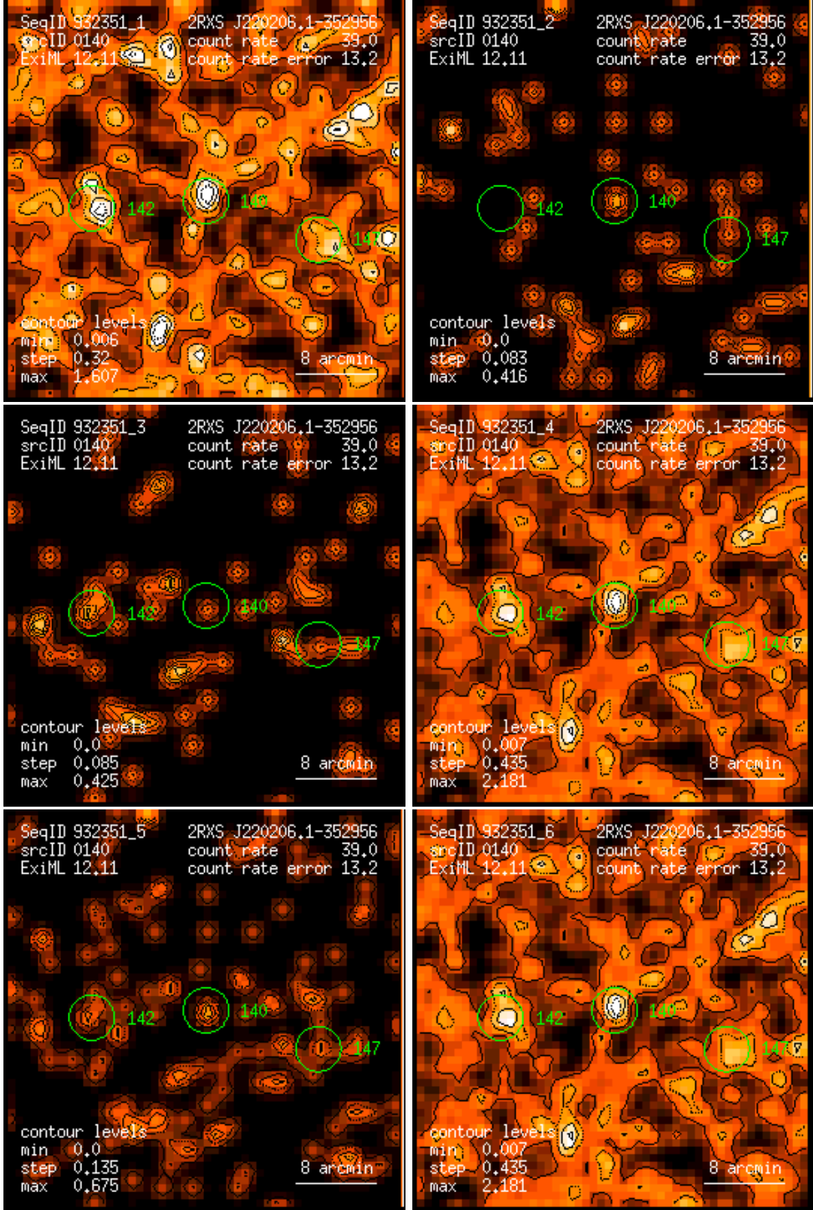
Figure 140: RASS 932351: detection 0140: band rate images, Gaussian filter: (1) PSPC channels 11 – 41, (2) 52 – 90, (3) 91 – 201, (4) 11 – 235, (5) 52 – 201, (6) 11 – 201. Broad band rates in counts/ks. Band rate contour levels in counts/ks/arcmin 2 .
