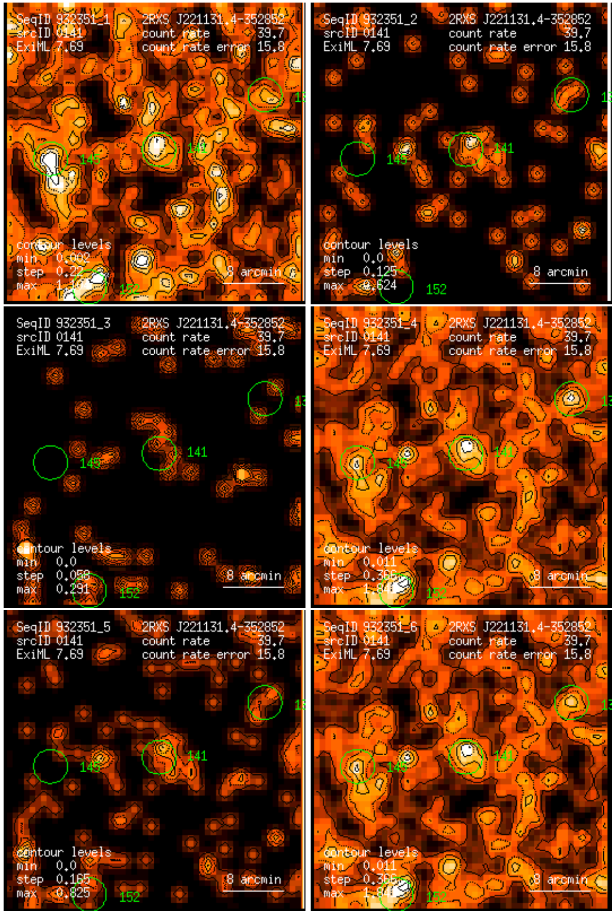
Figure 141: RASS 932351: detection 0141: band rate images, Gaussian filter: (1) PSPC channels 11 – 41, (2) 52 – 90, (3) 91 – 201, (4) 11 – 235, (5) 52 – 201, (6) 11 – 201. Broad band rates in counts/ks. Band rate contour levels in counts/ks/arcmin 2 .
