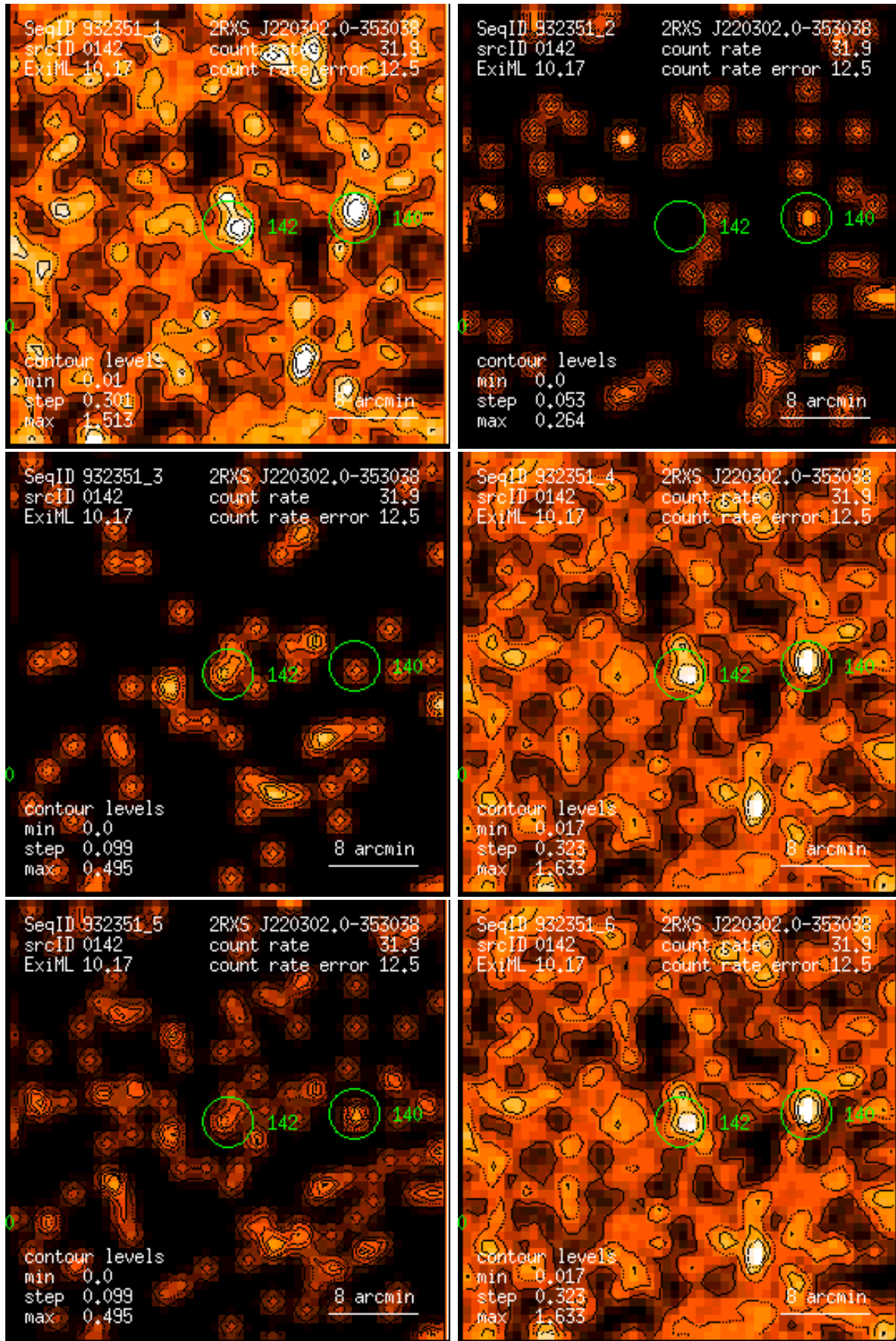
Figure 142: RASS 932351: detection 0142: band rate images, Gaussian filter: (1) PSPC channels 11 – 41, (2) 52 – 90, (3) 91 – 201, (4) 11 – 235, (5) 52 – 201, (6) 11 – 201. Broad band rates in counts/ks. Band rate contour levels in counts/ks/arcmin 2 .
