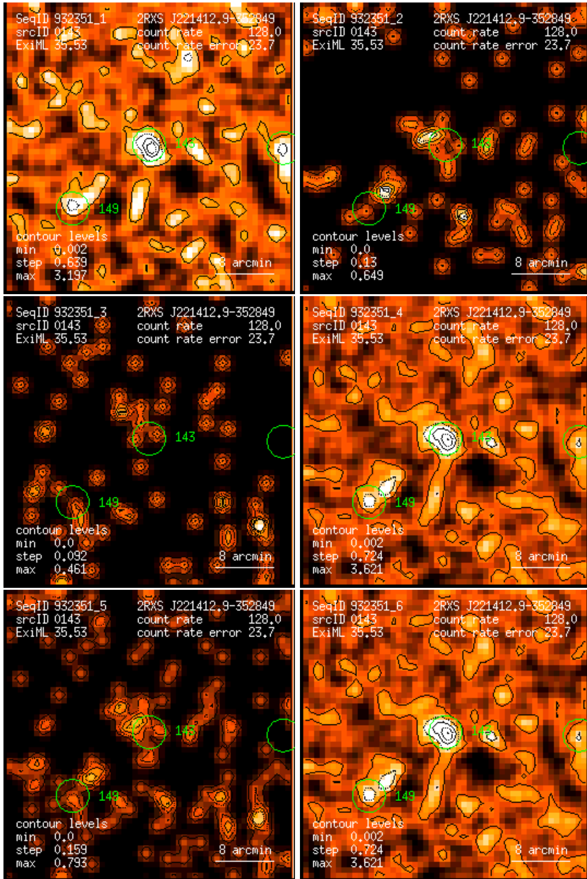
Figure 143: RASS 932351: detection 0143: band rate images, Gaussian filter: (1) PSPC channels 11 – 41, (2) 52 – 90, (3) 91 – 201, (4) 11 – 235, (5) 52 – 201, (6) 11 – 201. Broad band rates in counts/ks. Band rate contour levels in counts/ks/arcmin 2 .
