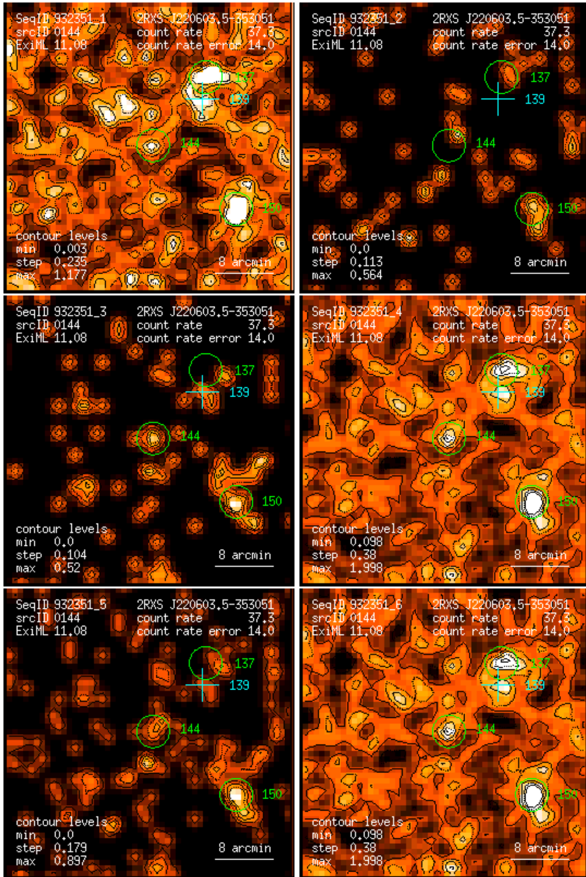
Figure 144: RASS 932351: detection 0144: band rate images, Gaussian filter: (1) PSPC channels 11 – 41, (2) 52 – 90, (3) 91 – 201, (4) 11 – 235, (5) 52 – 201, (6) 11 – 201. Broad band rates in counts/ks. Band rate contour levels in counts/ks/arcmin 2 .
