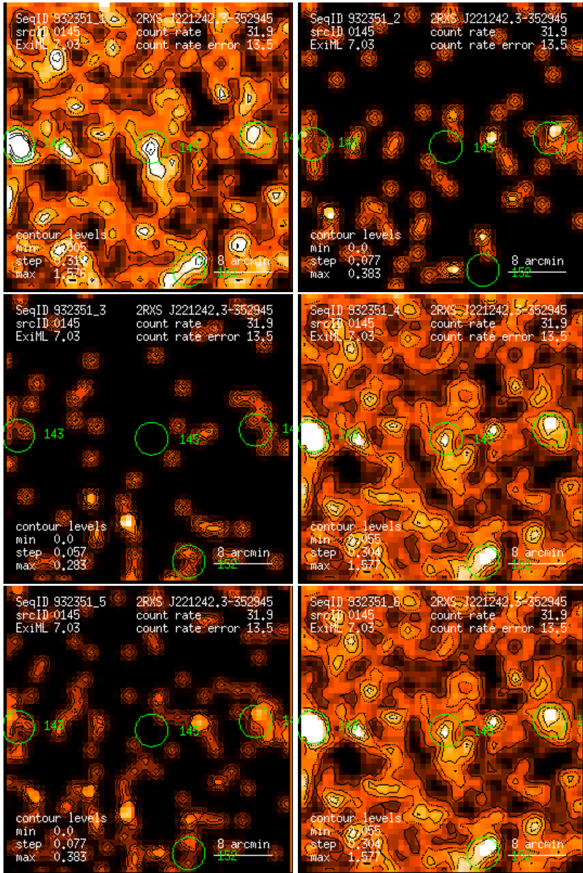
Figure 145: RASS 932351: detection 0145: band rate images, Gaussian filter: (1) PSPC channels 11 – 41, (2) 52 – 90, (3) 91 – 201, (4) 11 – 235, (5) 52 – 201, (6) 11 – 201. Broad band rates in counts/ks. Band rate contour levels in counts/ks/arcmin 2 .
