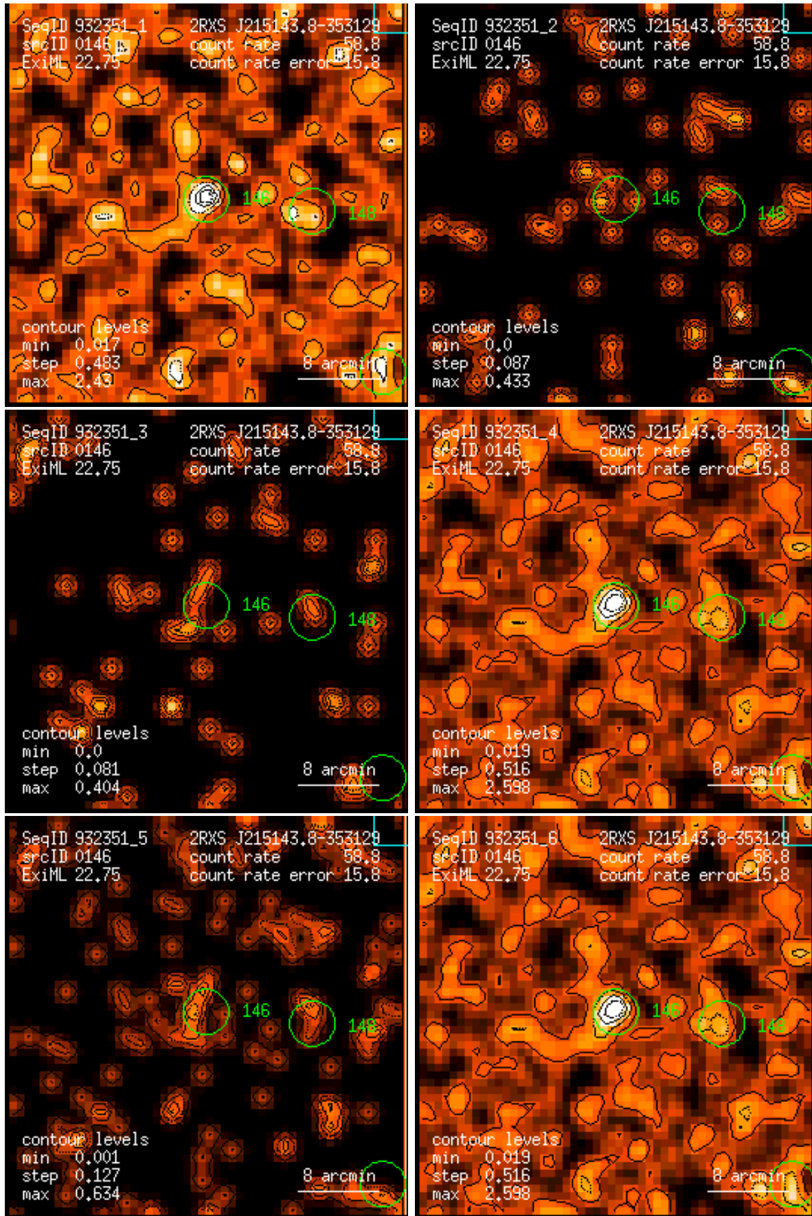
Figure 146: RASS 932351: detection 0146: band rate images, Gaussian filter: (1) PSPC channels 11 – 41, (2) 52 – 90, (3) 91 – 201, (4) 11 – 235, (5) 52 – 201, (6) 11 – 201. Broad band rates in counts/ks. Band rate contour levels in counts/ks/arcmin 2 .
