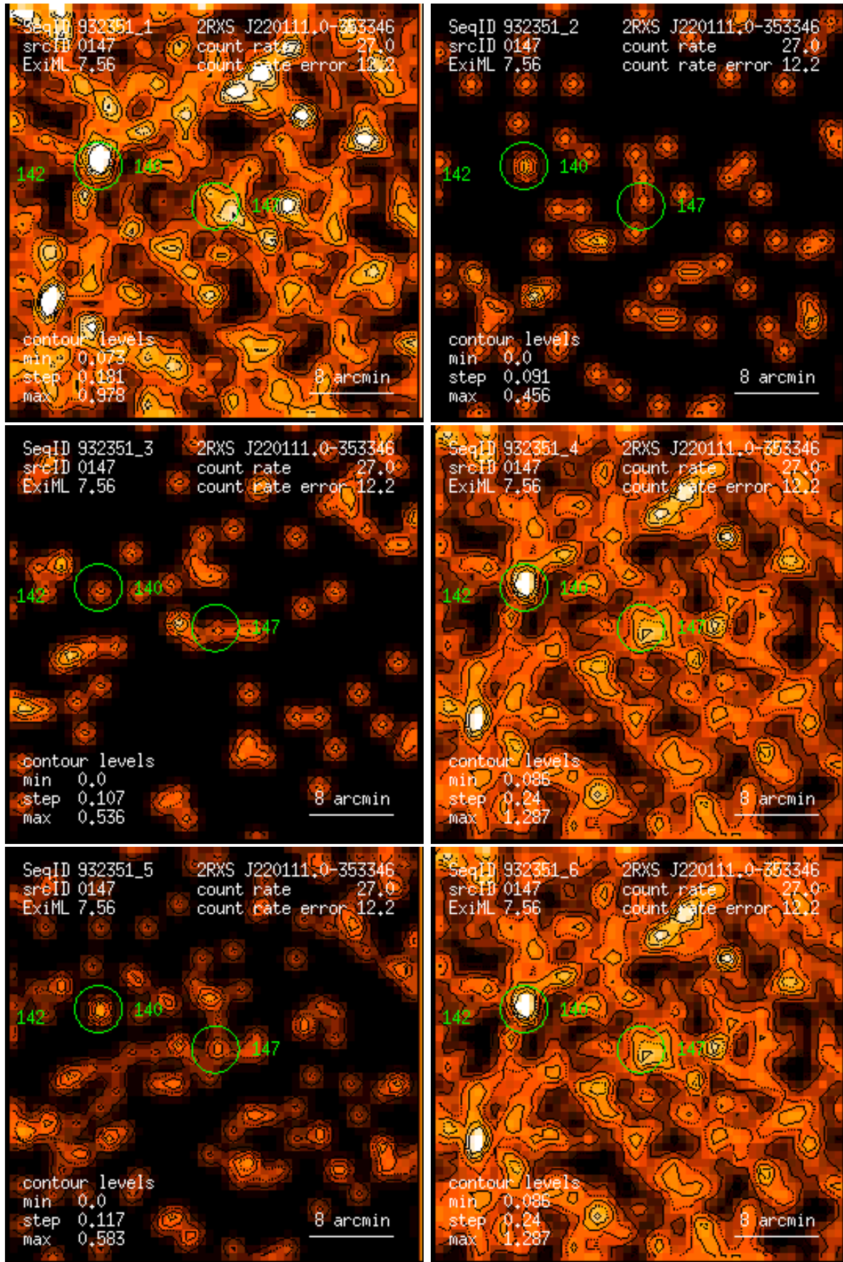
Figure 147: RASS 932351: detection 0147: band rate images, Gaussian filter: (1) PSPC channels 11 – 41, (2) 52 – 90, (3) 91 – 201, (4) 11 – 235, (5) 52 – 201, (6) 11 – 201. Broad band rates in counts/ks. Band rate contour levels in counts/ks/arcmin 2 .
