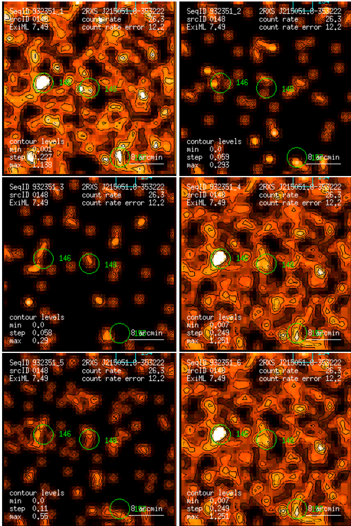
Figure 148: RASS 932351: detection 0148: band rate images, Gaussian filter: (1) PSPC channels 11 – 41, (2) 52 – 90, (3) 91 – 201, (4) 11 – 235, (5) 52 – 201, (6) 11 – 201. Broad band rates in counts/ks. Band rate contour levels in counts/ks/arcmin 2 .
