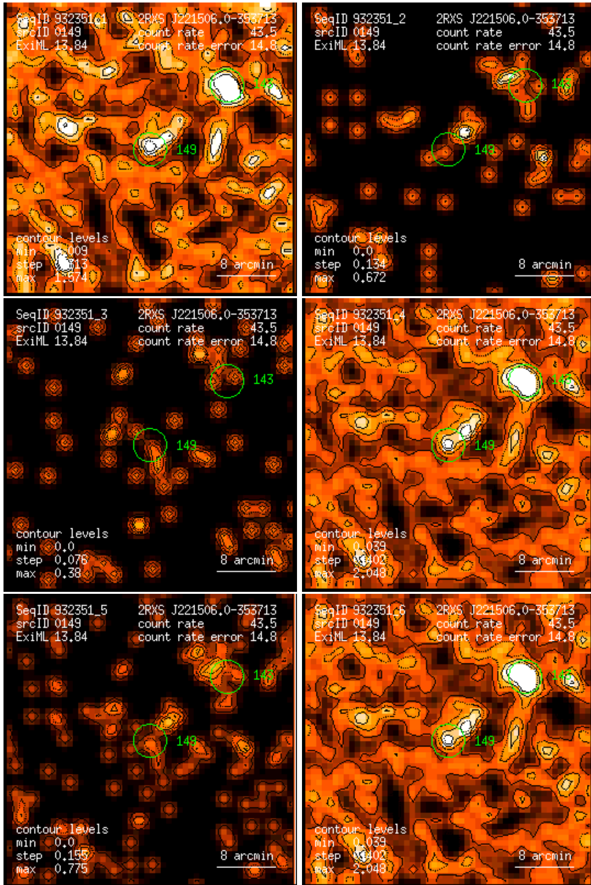
Figure 149: RASS 932351: detection 0149: band rate images, Gaussian filter: (1) PSPC channels 11 – 41, (2) 52 – 90, (3) 91 – 201, (4) 11 – 235, (5) 52 – 201, (6) 11 – 201. Broad band rates in counts/ks. Band rate contour levels in counts/ks/arcmin 2 .
