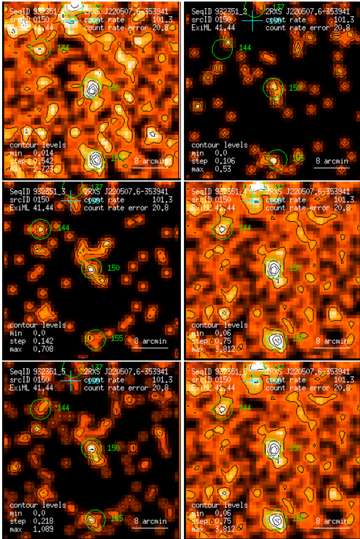
Figure 150: RASS 932351: detection 0150: band rate images, Gaussian filter: (1) PSPC channels 11 – 41, (2) 52 – 90, (3) 91 – 201, (4) 11 – 235, (5) 52 – 201, (6) 11 – 201. Broad band rates in counts/ks. Band rate contour levels in counts/ks/arcmin 2 .
