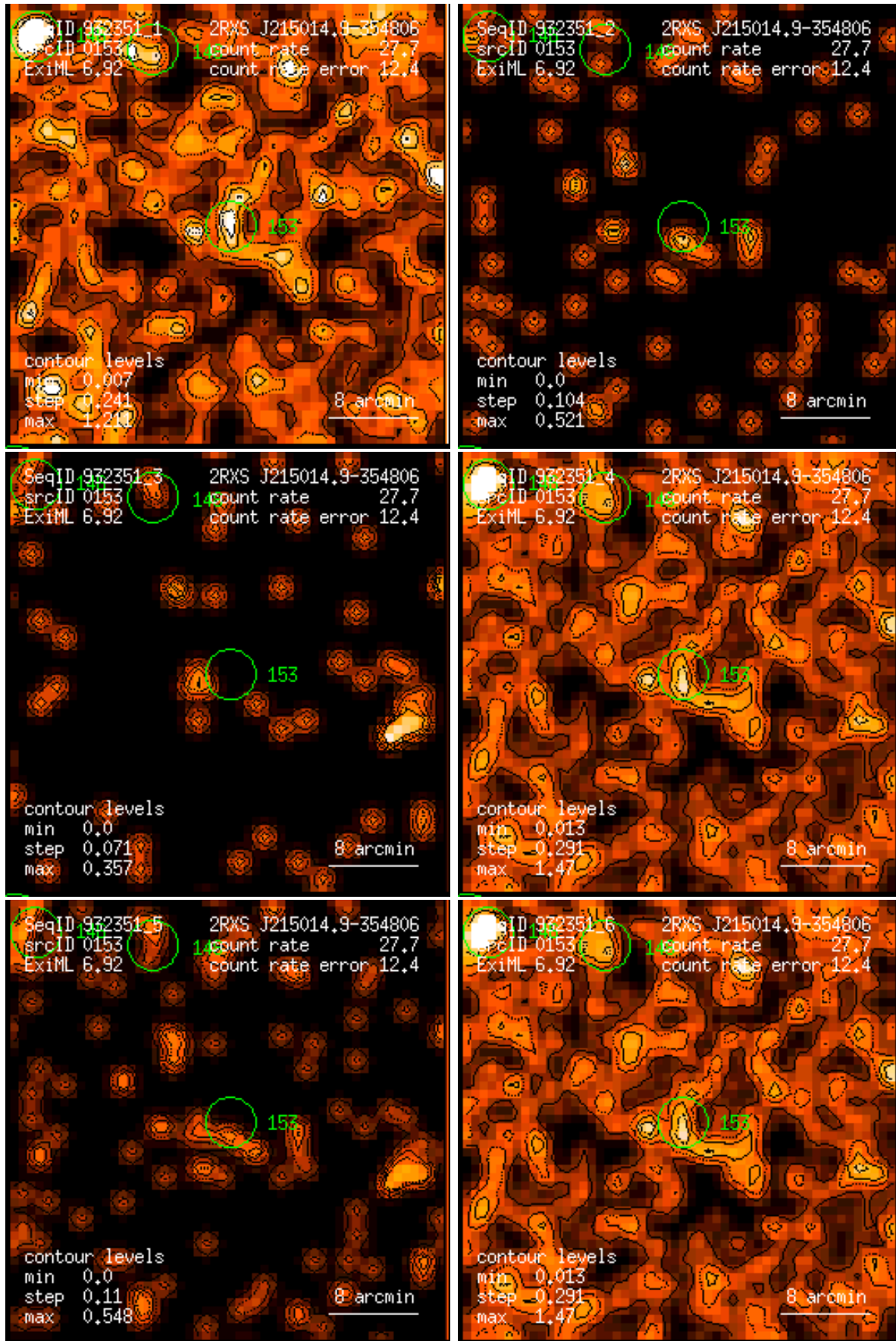
Figure 153: RASS 932351: detection 0153: band rate images, Gaussian filter: (1) PSPC channels 11 – 41, (2) 52 – 90, (3) 91 – 201, (4) 11 – 235, (5) 52 – 201, (6) 11 – 201. Broad band rates in counts/ks. Band rate contour levels in counts/ks/arcmin 2 .
