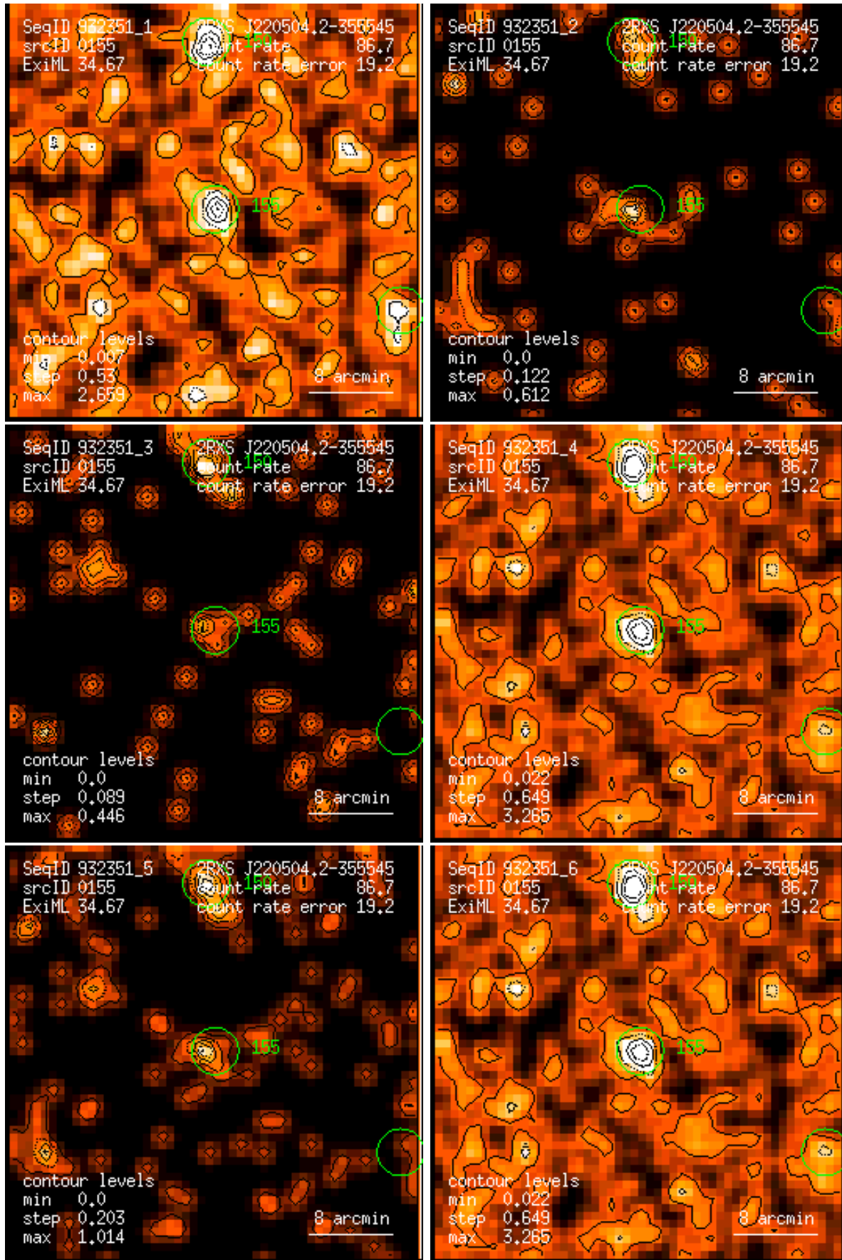
Figure 155: RASS 932351: detection 0155: band rate images, Gaussian filter: (1) PSPC channels 11 – 41, (2) 52 – 90, (3) 91 – 201, (4) 11 – 235, (5) 52 – 201, (6) 11 – 201. Broad band rates in counts/ks. Band rate contour levels in counts/ks/arcmin 2 .
