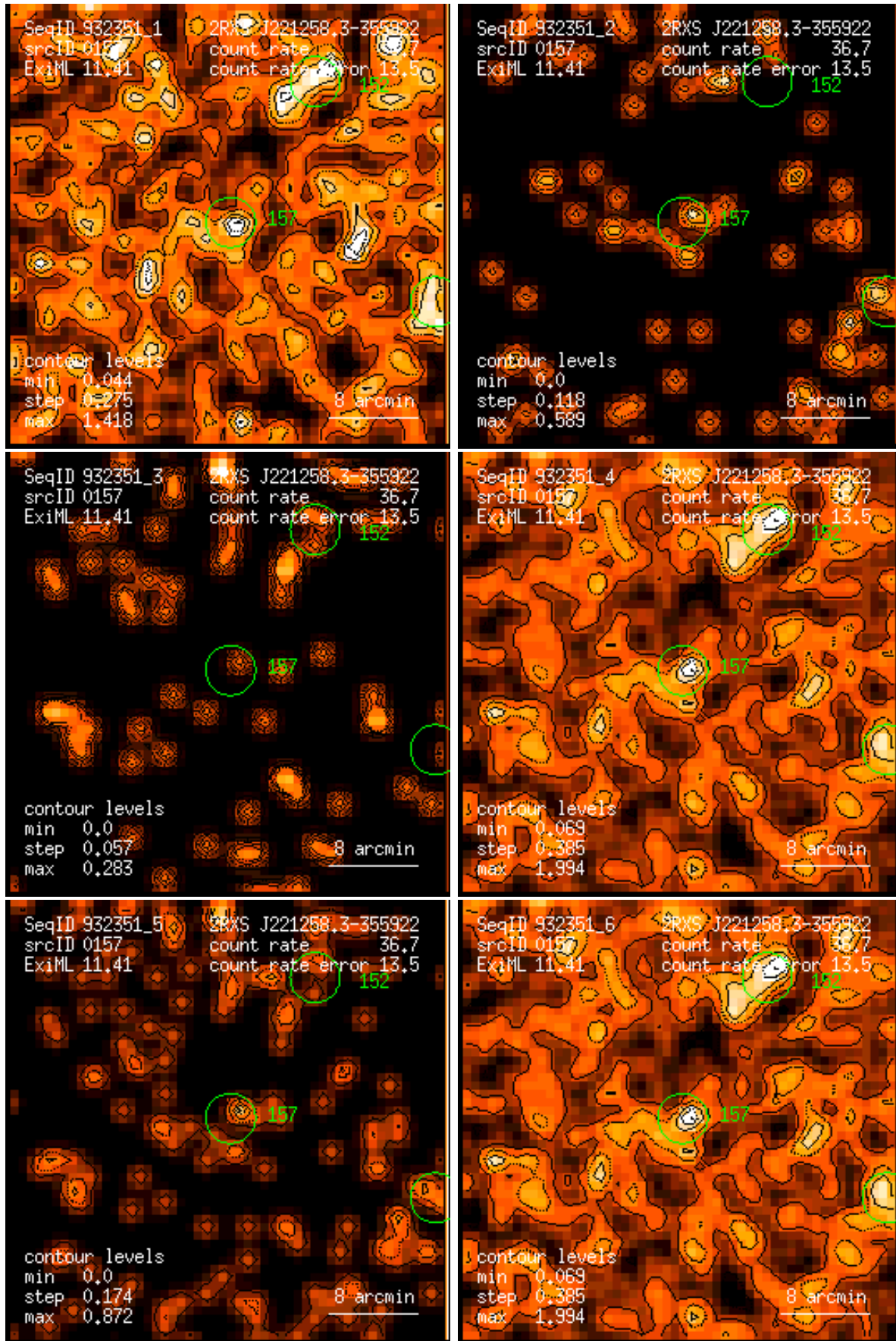
Figure 157: RASS 932351: detection 0157: band rate images, Gaussian filter: (1) PSPC channels 11 – 41, (2) 52 – 90, (3) 91 – 201, (4) 11 – 235, (5) 52 – 201, (6) 11 – 201. Broad band rates in counts/ks. Band rate contour levels in counts/ks/arcmin 2 .
