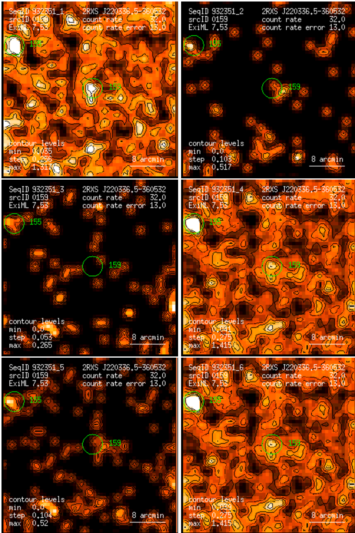
Figure 159: RASS 932351: detection 0159: band rate images, Gaussian filter: (1) PSPC channels 11 – 41, (2) 52 – 90, (3) 91 – 201, (4) 11 – 235, (5) 52 – 201, (6) 11 – 201. Broad band rates in counts/ks. Band rate contour levels in counts/ks/arcmin 2 .
