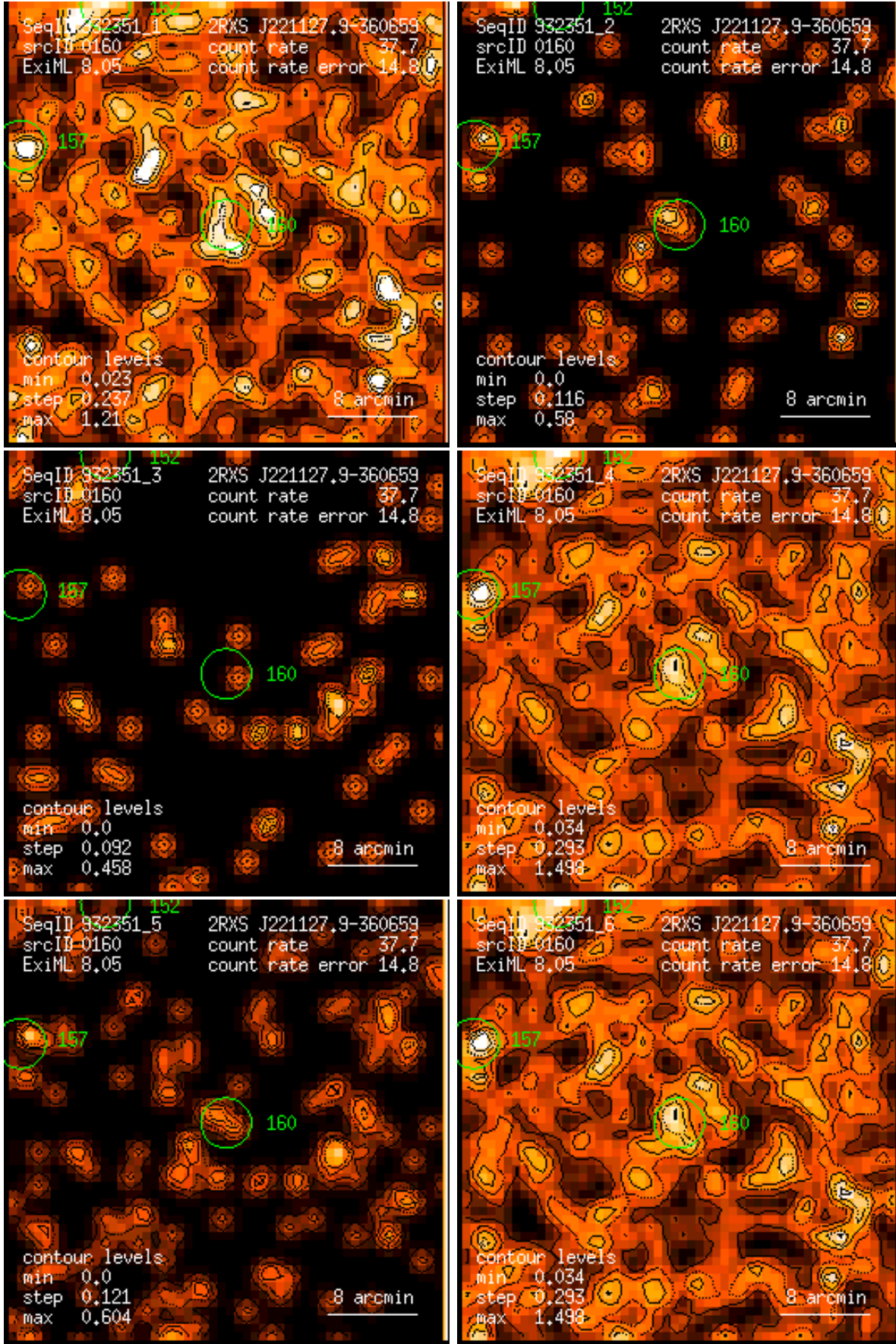
Figure 160: RASS 932351: detection 0160: band rate images, Gaussian filter: (1) PSPC channels 11 – 41, (2) 52 – 90, (3) 91 – 201, (4) 11 – 235, (5) 52 – 201, (6) 11 – 201. Broad band rates in counts/ks. Band rate contour levels in counts/ks/arcmin 2 .
