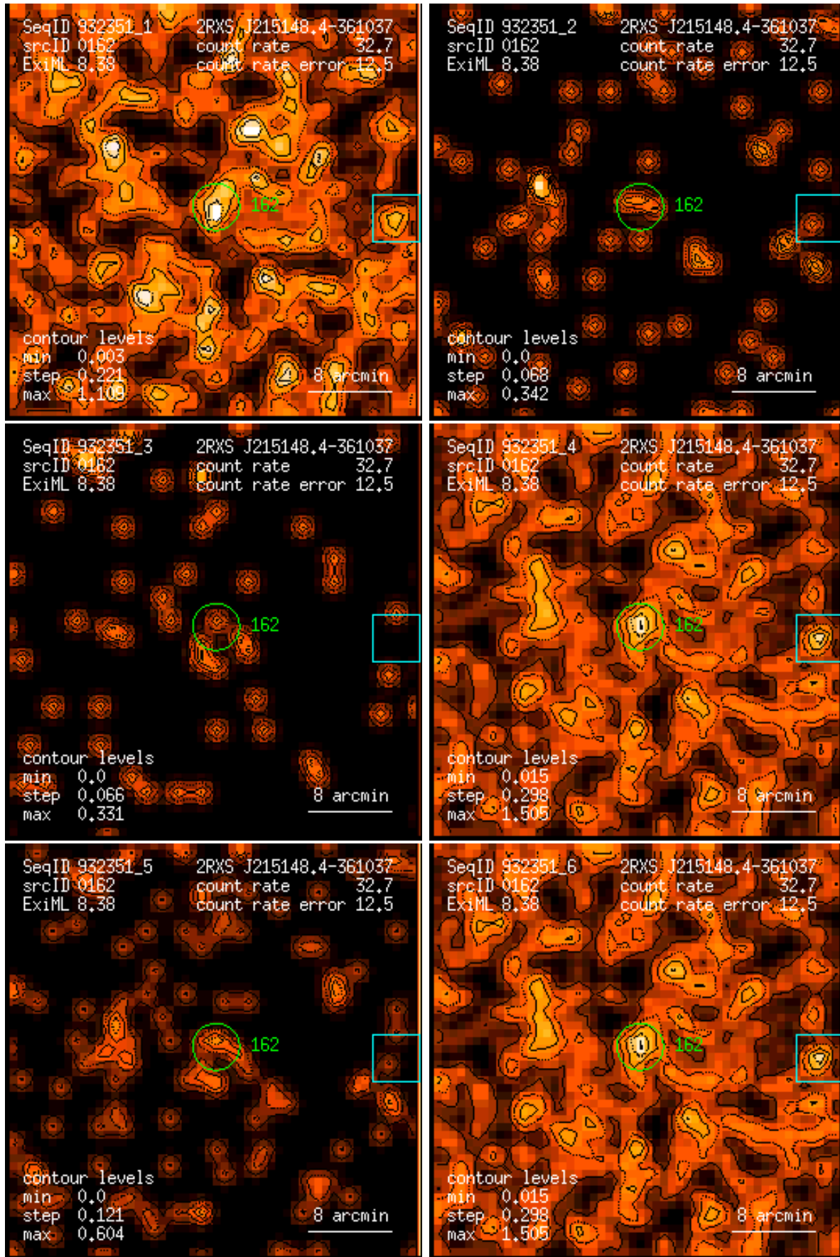
Figure 162: RASS 932351: detection 0162: band rate images, Gaussian filter: (1) PSPC channels 11 – 41, (2) 52 – 90, (3) 91 – 201, (4) 11 – 235, (5) 52 – 201, (6) 11 – 201. Broad band rates in counts/ks. Band rate contour levels in counts/ks/arcmin 2 .
