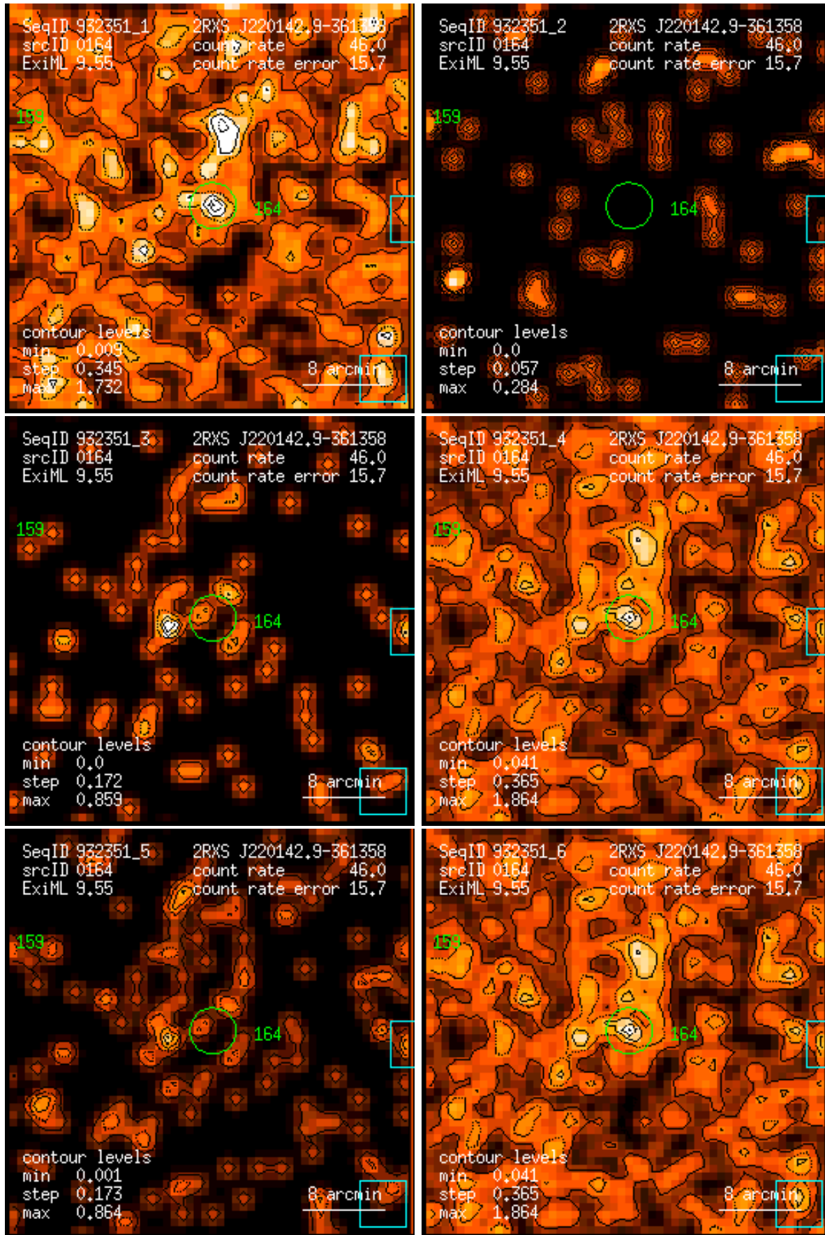
Figure 164: RASS 932351: detection 0164: band rate images, Gaussian filter: (1) PSPC channels 11 – 41, (2) 52 – 90, (3) 91 – 201, (4) 11 – 235, (5) 52 – 201, (6) 11 – 201. Broad band rates in counts/ks. Band rate contour levels in counts/ks/arcmin 2 .
