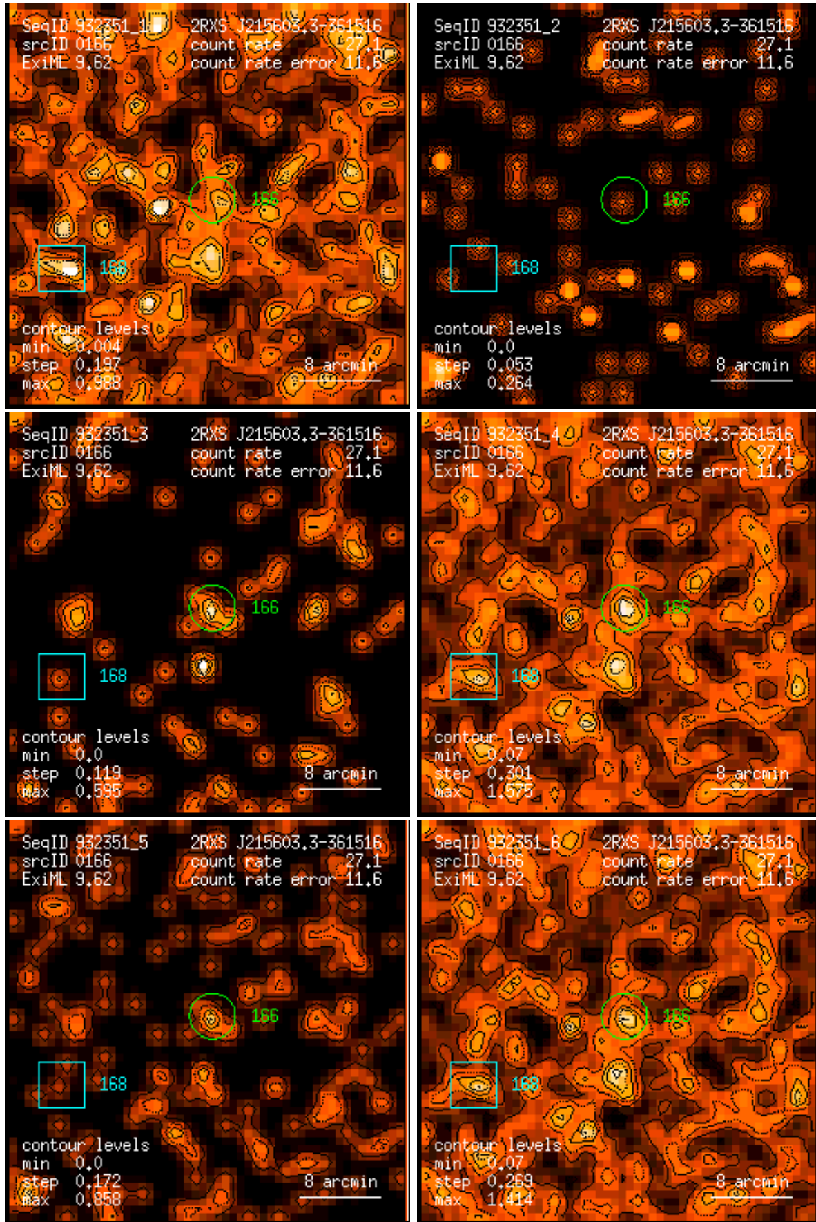
Figure 166: RASS 932351: detection 0166: band rate images, Gaussian filter: (1) PSPC channels 11 – 41, (2) 52 – 90, (3) 91 – 201, (4) 11 – 235, (5) 52 – 201, (6) 11 – 201. Broad band rates in counts/ks. Band rate contour levels in counts/ks/arcmin 2 .
