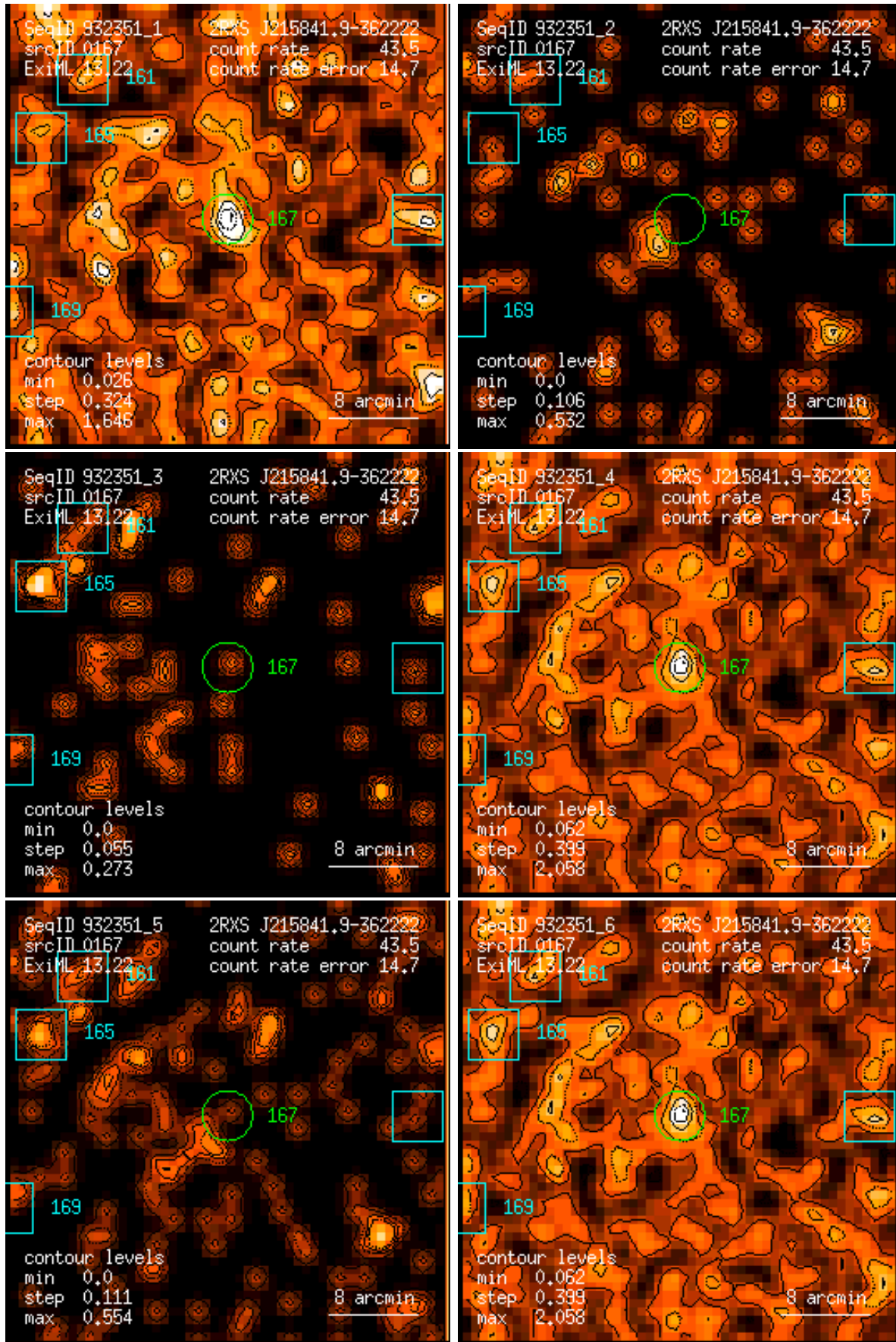
Figure 167: RASS 932351: detection 0167: band rate images, Gaussian filter: (1) PSPC channels 11 – 41, (2) 52 – 90, (3) 91 – 201, (4) 11 – 235, (5) 52 – 201, (6) 11 – 201. Broad band rates in counts/ks. Band rate contour levels in counts/ks/arcmin 2 .
