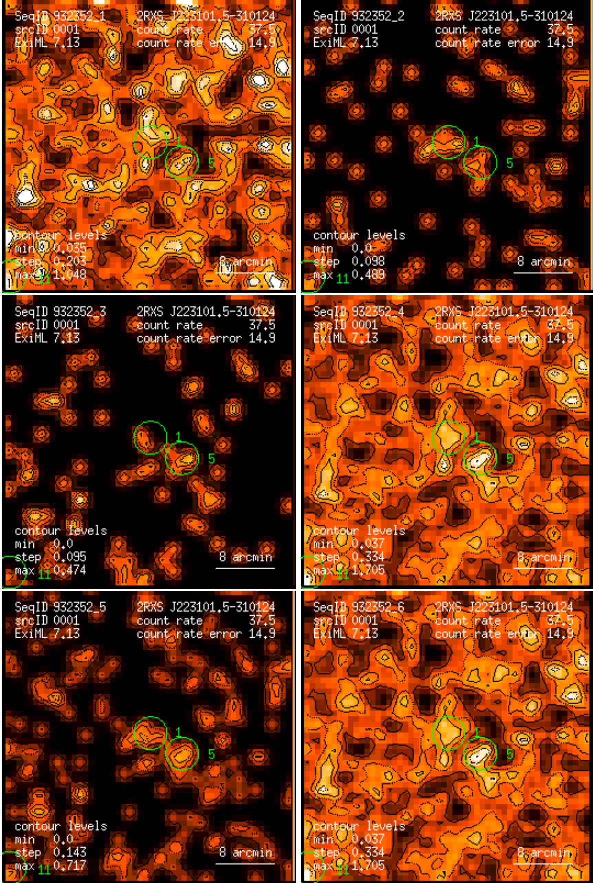
Figure 1: RASS 932352: detection 0001: band rate images, Gaussian filter: (1) PSPC channels 11 – 41, (2) 52 – 90, (3) 91 – 201, (4) 11 – 235, (5) 52 – 201, (6) 11 – 201. Broad band rates in counts/ks. Band rate contour levels in counts/ks/arcmin 2 .
