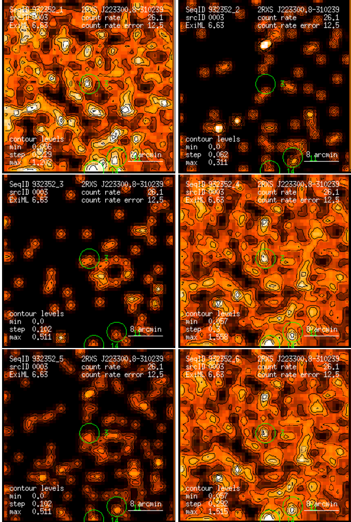
Figure 3: RASS 932352: detection 0003: band rate images, Gaussian filter: (1) PSPC channels 11 – 41, (2) 52 – 90, (3) 91 – 201, (4) 11 – 235, (5) 52 – 201, (6) 11 – 201. Broad band rates in counts/ks. Band rate contour levels in counts/ks/arcmin 2 .
