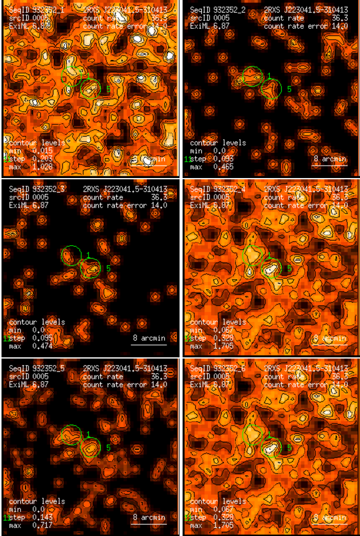
Figure 5: RASS 932352: detection 0005: band rate images, Gaussian filter: (1) PSPC channels 11 – 41, (2) 52 – 90, (3) 91 – 201, (4) 11 – 235, (5) 52 – 201, (6) 11 – 201. Broad band rates in counts/ks. Band rate contour levels in counts/ks/arcmin 2 .
