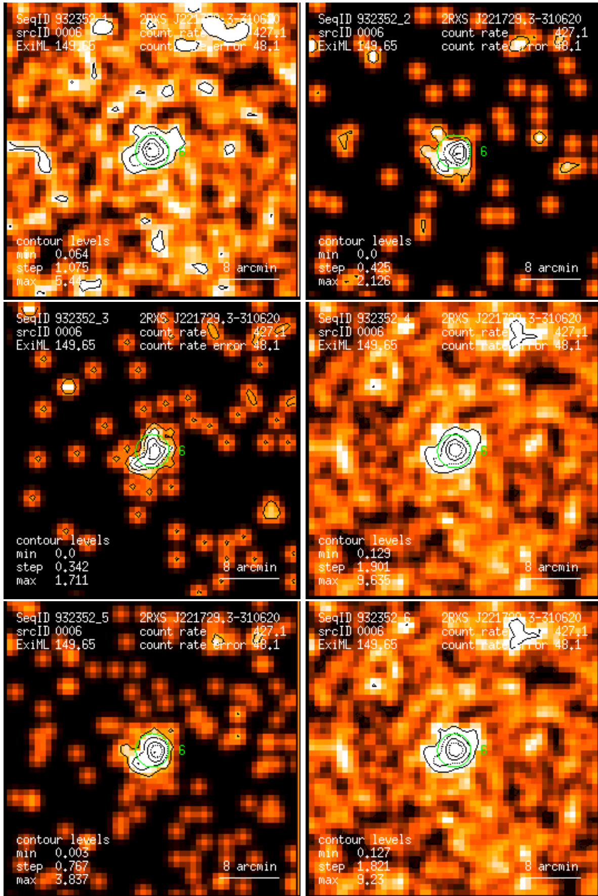
Figure 6: RASS 932352: detection 0006: band rate images, Gaussian filter: (1) PSPC channels 11 – 41, (2) 52 – 90, (3) 91 – 201, (4) 11 – 235, (5) 52 – 201, (6) 11 – 201. Broad band rates in counts/ks. Band rate contour levels in counts/ks/arcmin 2 .
