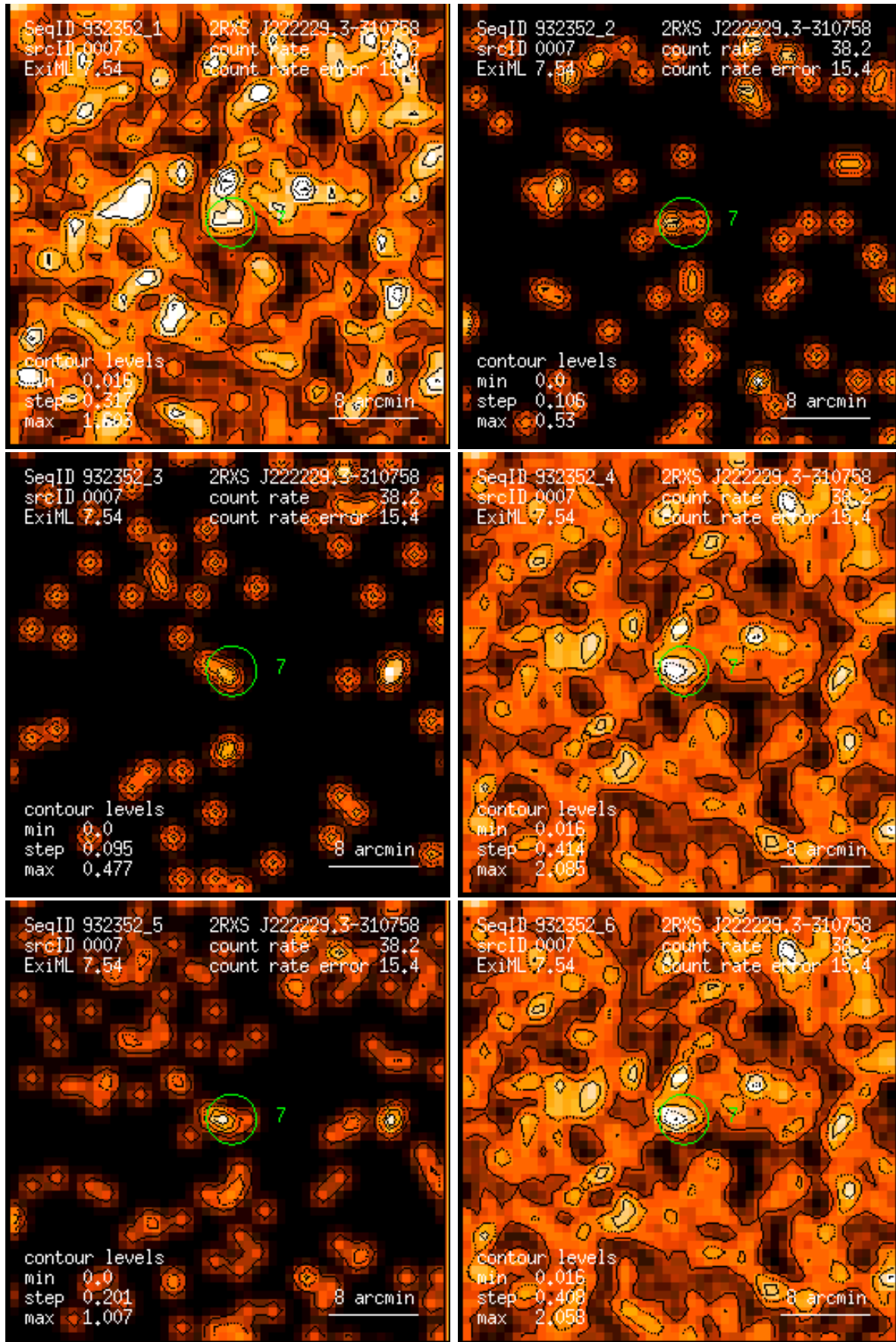
Figure 7: RASS 932352: detection 0007: band rate images, Gaussian filter: (1) PSPC channels 11 – 41, (2) 52 – 90, (3) 91 – 201, (4) 11 – 235, (5) 52 – 201, (6) 11 – 201. Broad band rates in counts/ks. Band rate contour levels in counts/ks/arcmin 2 .
