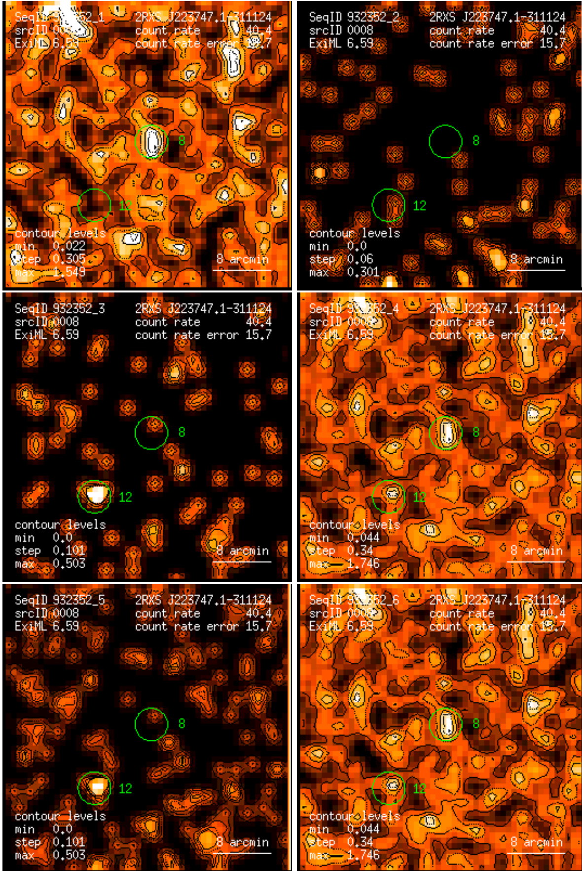
Figure 8: RASS 932352: detection 0008: band rate images, Gaussian filter: (1) PSPC channels 11 – 41, (2) 52 – 90, (3) 91 – 201, (4) 11 – 235, (5) 52 – 201, (6) 11 – 201. Broad band rates in counts/ks. Band rate contour levels in counts/ks/arcmin 2 .
