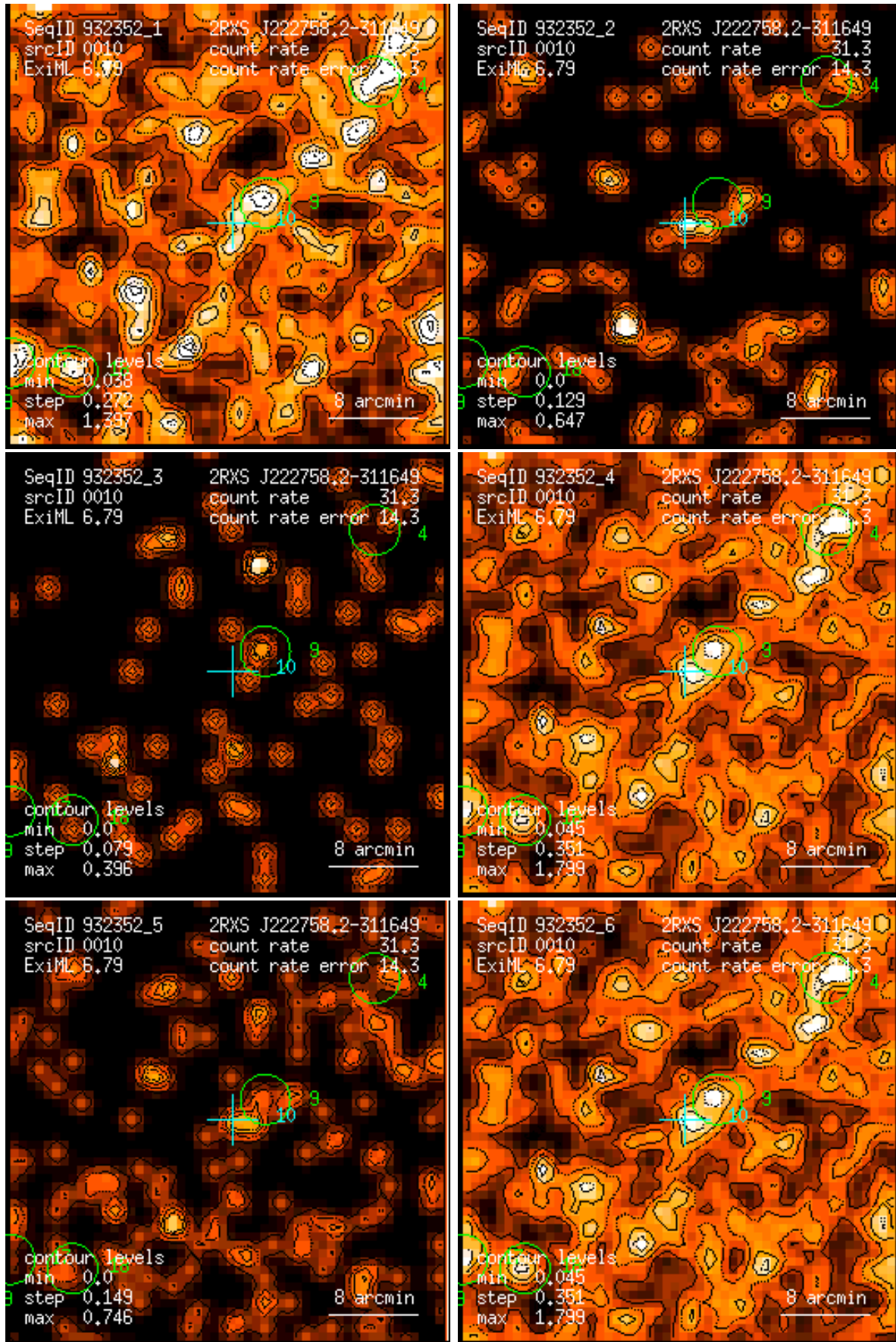
Figure 10: RASS 932352: detection 0010: band rate images, Gaussian filter: (1) PSPC channels 11 – 41, (2) 52 – 90, (3) 91 – 201, (4) 11 – 235, (5) 52 – 201, (6) 11 – 201. Broad band rates in counts/ks. Band rate contour levels in counts/ks/arcmin 2 .
