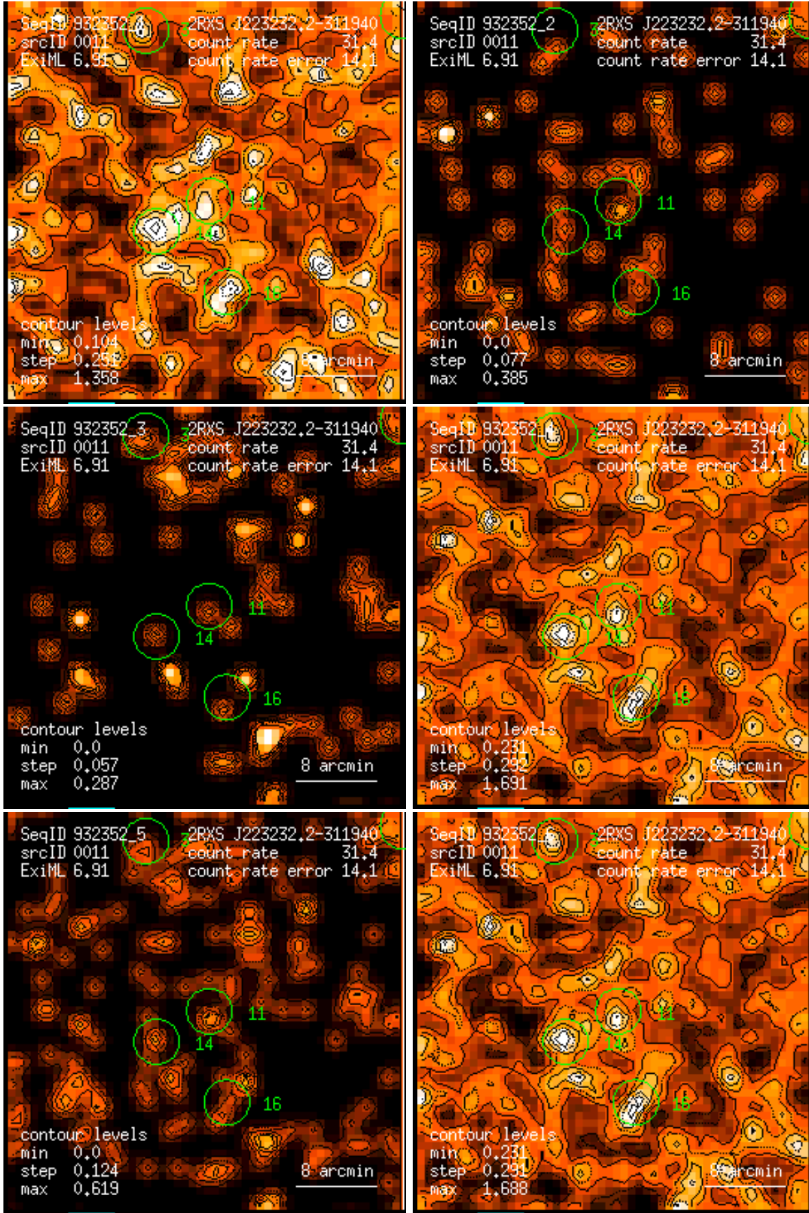
Figure 11: RASS 932352: detection 0011: band rate images, Gaussian filter: (1) PSPC channels 11 – 41, (2) 52 – 90, (3) 91 – 201, (4) 11 – 235, (5) 52 – 201, (6) 11 – 201. Broad band rates in counts/ks. Band rate contour levels in counts/ks/arcmin 2 .
