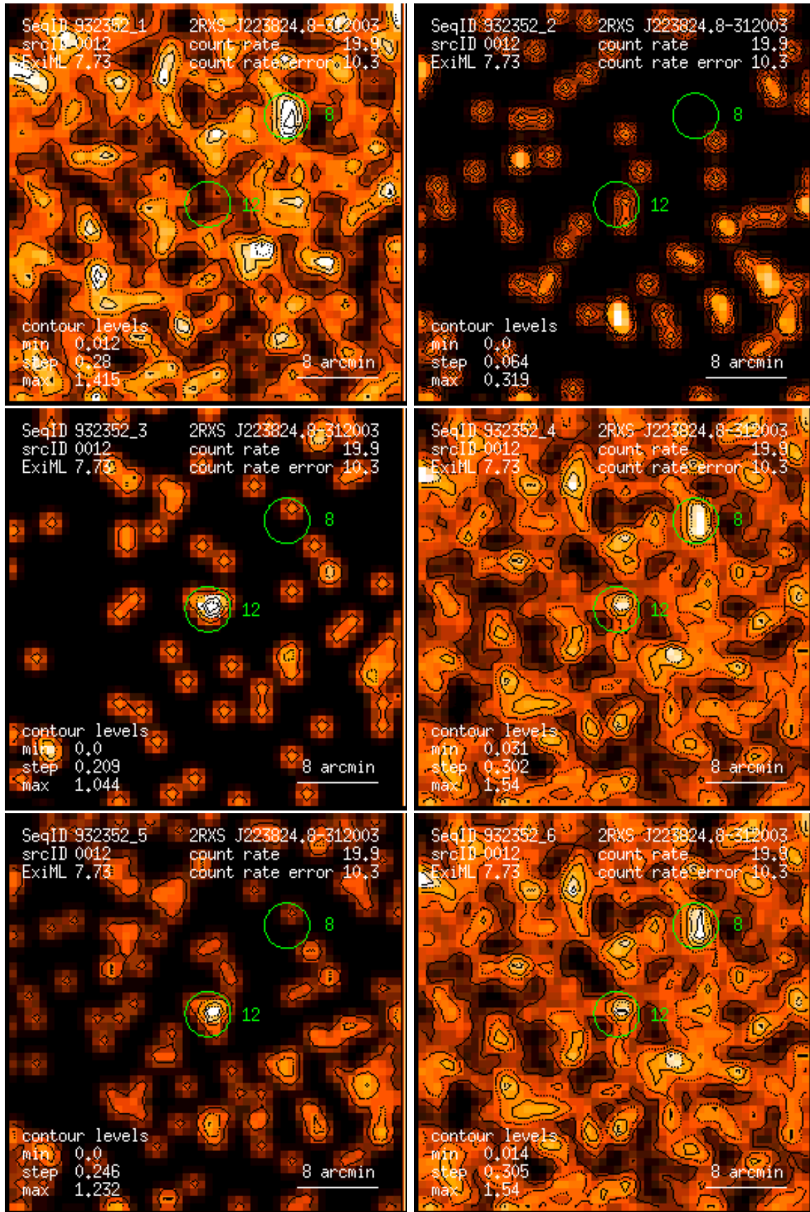
Figure 12: RASS 932352: detection 0012: band rate images, Gaussian filter: (1) PSPC channels 11 – 41, (2) 52 – 90, (3) 91 – 201, (4) 11 – 235, (5) 52 – 201, (6) 11 – 201. Broad band rates in counts/ks. Band rate contour levels in counts/ks/arcmin 2 .
