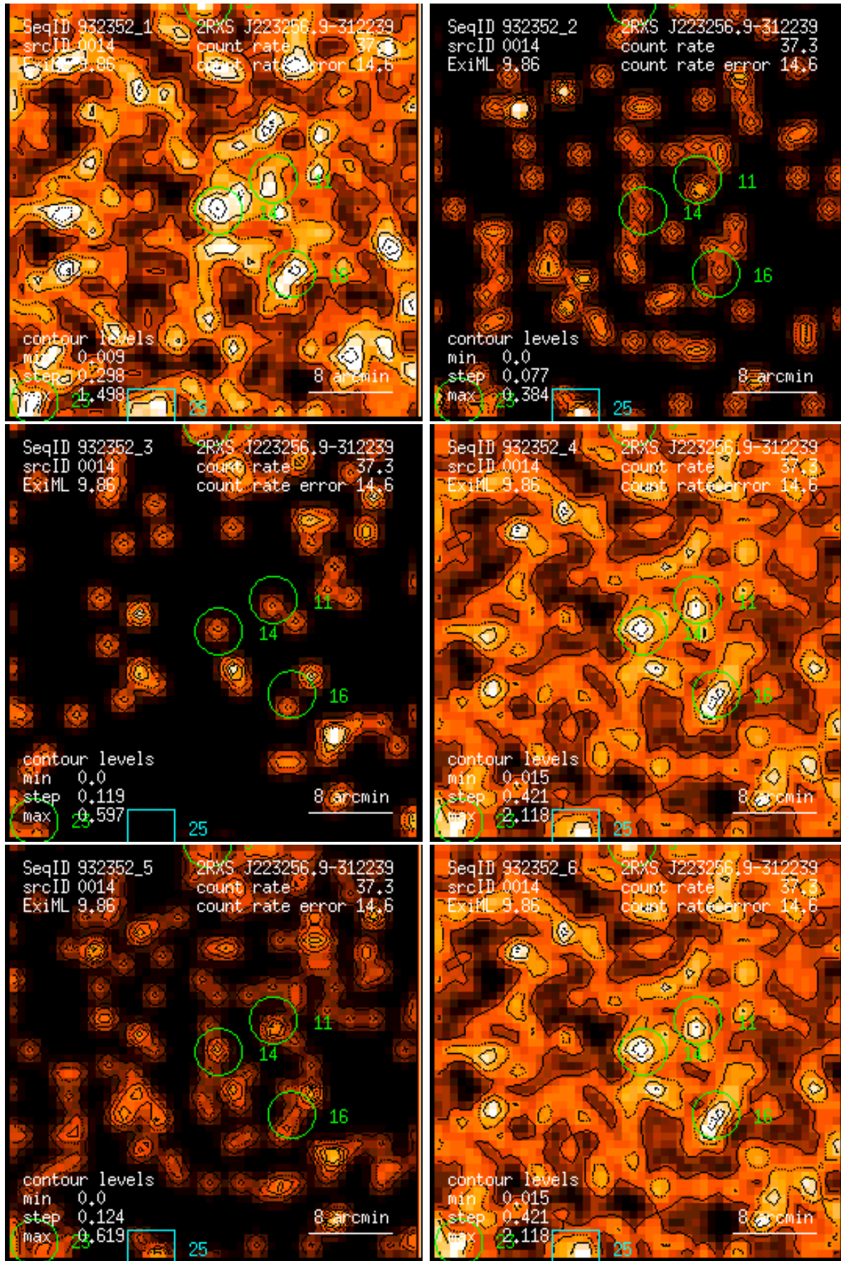
Figure 14: RASS 932352: detection 0014: band rate images, Gaussian filter: (1) PSPC channels 11 – 41, (2) 52 – 90, (3) 91 – 201, (4) 11 – 235, (5) 52 – 201, (6) 11 – 201. Broad band rates in counts/ks. Band rate contour levels in counts/ks/arcmin 2 .
