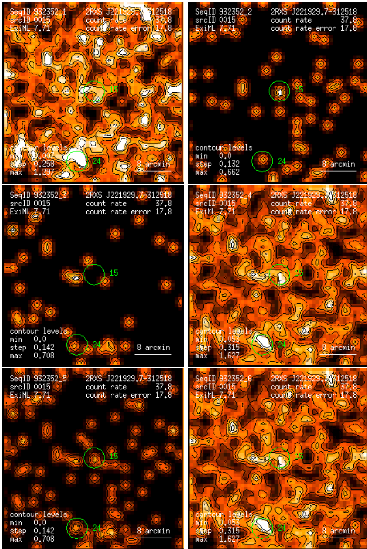
Figure 15: RASS 932352: detection 0015: band rate images, Gaussian filter: (1) PSPC channels 11 – 41, (2) 52 – 90, (3) 91 – 201, (4) 11 – 235, (5) 52 – 201, (6) 11 – 201. Broad band rates in counts/ks. Band rate contour levels in counts/ks/arcmin 2 .
