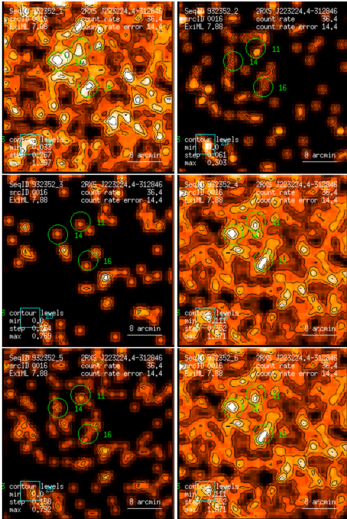
Figure 16: RASS 932352: detection 0016: band rate images, Gaussian filter: (1) PSPC channels 11 – 41, (2) 52 – 90, (3) 91 – 201, (4) 11 – 235, (5) 52 – 201, (6) 11 – 201. Broad band rates in counts/ks. Band rate contour levels in counts/ks/arcmin 2 .
