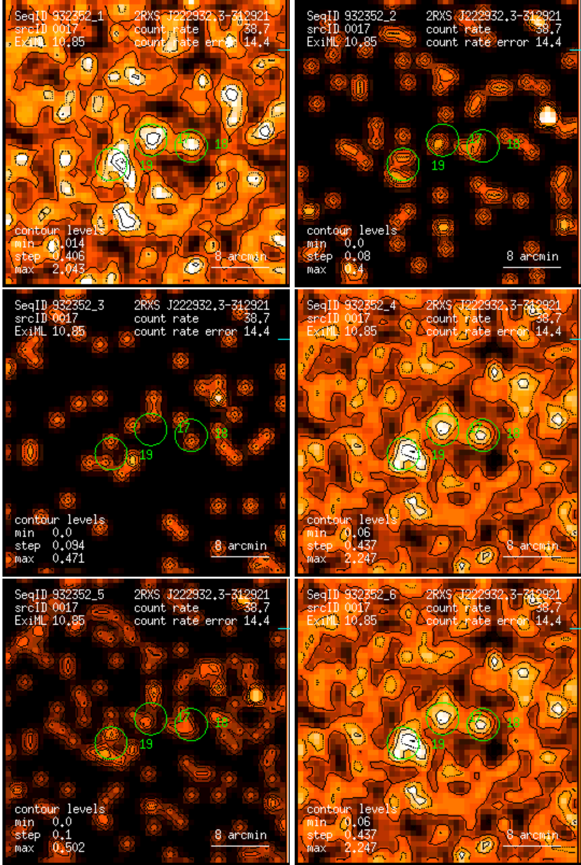
Figure 17: RASS 932352: detection 0017: band rate images, Gaussian filter: (1) PSPC channels 11 – 41, (2) 52 – 90, (3) 91 – 201, (4) 11 – 235, (5) 52 – 201, (6) 11 – 201. Broad band rates in counts/ks. Band rate contour levels in counts/ks/arcmin 2 .
