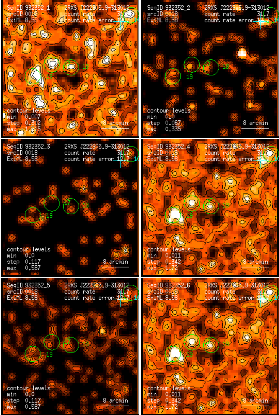
Figure 18: RASS 932352: detection 0018: band rate images, Gaussian filter: (1) PSPC channels 11 – 41, (2) 52 – 90, (3) 91 – 201, (4) 11 – 235, (5) 52 – 201, (6) 11 – 201. Broad band rates in counts/ks. Band rate contour levels in counts/ks/arcmin 2 .
